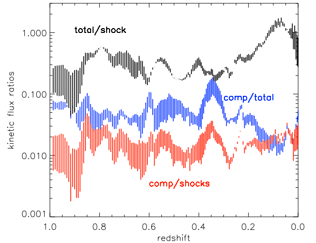
Figure 15. Evolution of different energy fluxes for it903 (averaged within the central 1.44^3 \text{ Mpc}^3 region: (a) total kinetic energy flux over shock kinetic power (black); (b) compressive kinetic energy flux over total kinetic energy flux (blue); (c) compressive kinetic energy flux over shock kinetic power (red). The spread in the ratios at each redshift indicates ranges related to the inclusion or exclusion of shocked regions to compute the kinetic energy flux (the upper bounds being the estimates including shocked regions).
