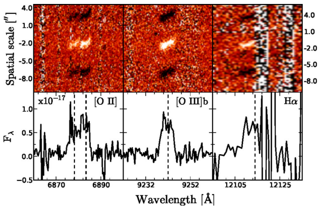
Figure 2. [O II], [O III]λ5007 and H \alpha lines as observed by the X-Shooter for GRB 000210 host. Both 2D (up) as well as extracted 1D (bottom) spectra are plotted for each line. In general, spatial and wavelength scale of VIS and NIR differ. Vertical dashed lines show redshifted air wavelengths of corresponding lines. Flux calibration of 1D spectra is not scaled with respect to photometric measurements or telluric stars (see Section 2).
