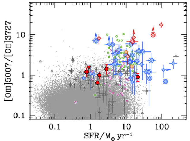
Figure 6. Dependence of [\text{O III}]\lambda 5007/[\text{O II}] on SFR for our six hosts (red points, triangle marks an upper limit for the host of GRB 000911). Also plotted are data from Nakajima & Ouchi (2014): SDSS galaxies (grey points); red and blue diamonds represent z = 2-3 Lyman \alpha emitters and Lyman-break galaxies, respectively (diamonds with circles denote z > 3 galaxies); grey triangles are z \sim 1 star-forming galaxies; green and purple circles show Green Pea galaxies and Lyman break analogues, while the orange pentagons are Lyman continuum leakers in the Local Universe. To convert our SFR values to Chabrier (2003) IMF, we multiplied them by a factor of 1.2.
