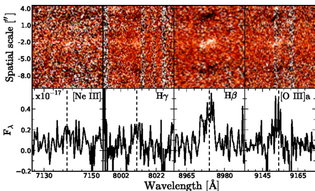
Figure 3. [Ne III], H \gamma , H \beta and [O III]λ4959 lines as observed by the X-Shooter for GRB 000210 host.
