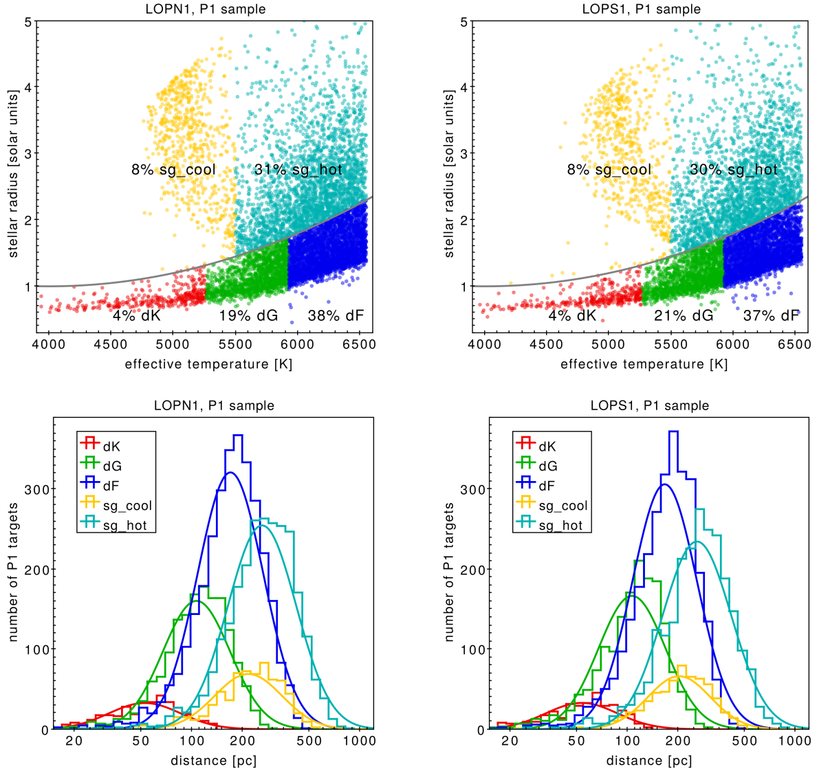
Fig. 9. Astrophysical parameters of the P1 targets within the LOPN1 ( left panels ) and LOPS1 ( right panels ) provisional fields. Top panels: Distribution of P1 targets on the (T_{\text{eff}}, R_*) plane; stars are classified into five distinct groups representing main-sequence K-type dwarfs (dK), G dwarfs (dG), F dwarfs (dF), subgiants at T_{\text{eff}} < 5500 K (sg_cool), and T_{\text{eff}} > 5500 K (sg_hot). The labels show their relative occurrence. The gray line in both panels marks an arbitrary boundary between main-sequence and evolved stars (see text). Bottom panels: Histograms of the distribution in distance of the same subgroups. The best-fit lognormal distribution is also over-plotted with a continuous line.
