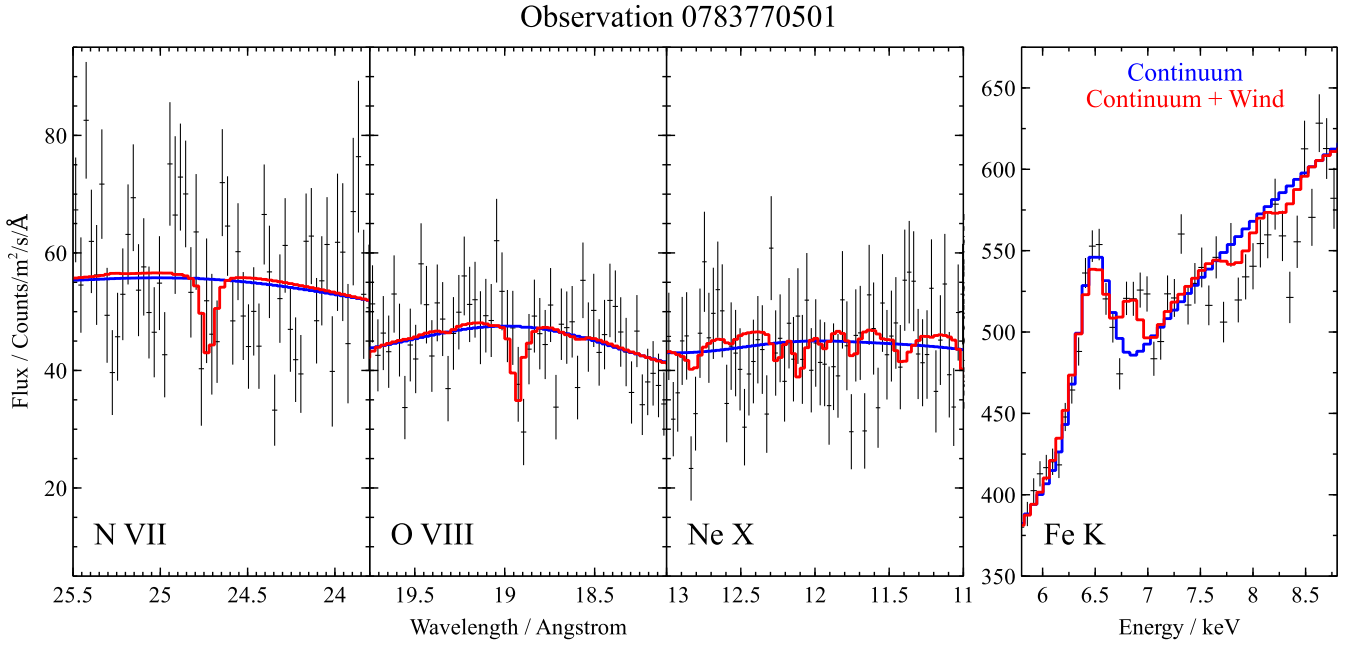
Figure 6. Same plot as Fig. 3 but for observation 0783770501.
