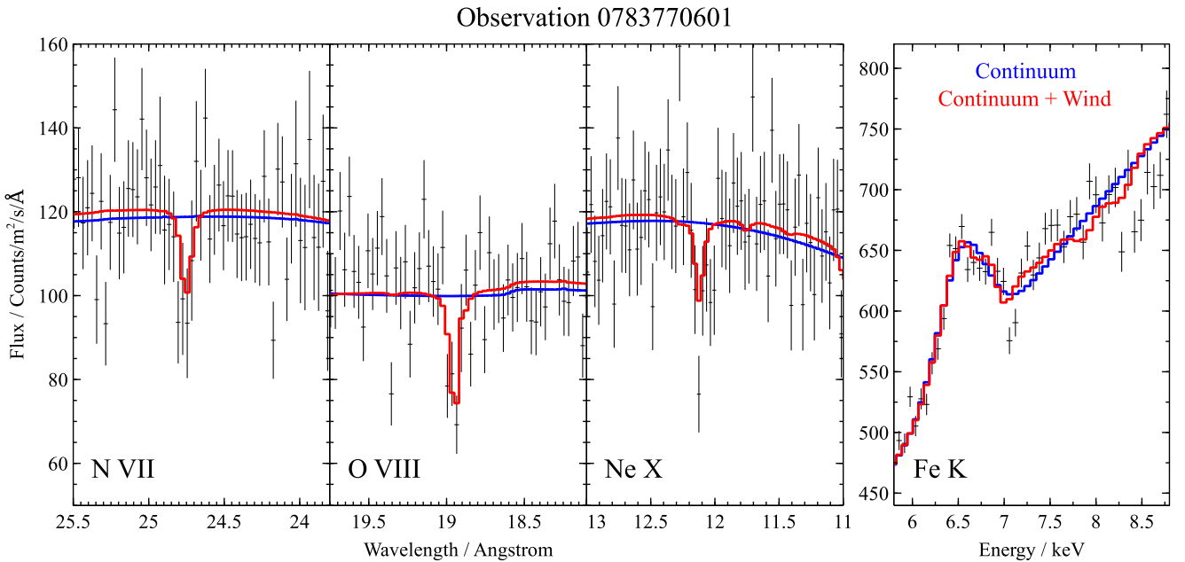
Figure 7. Same plot as Fig. 3 but for observation 0783770601.
