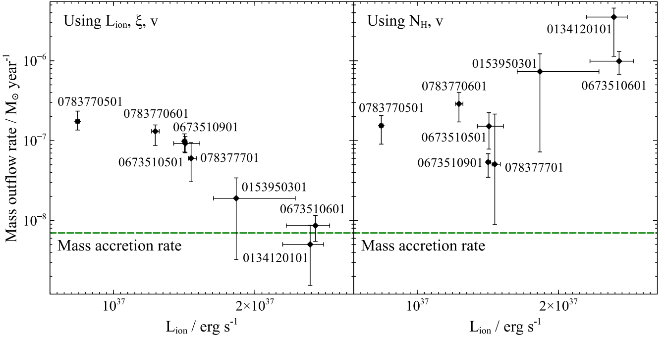
Figure 13. The mass outflow rate of the wind for each observation. The estimate in the left-hand plot was made using the ionizing luminosity of the source, the ionization parameter, and the velocity of the material. The estimate in the right-hand plot was made using the column density and the velocity of the wind. The green horizontal lines show the mass accretion rate through the accretion disc (Boroson et al. 2007).
