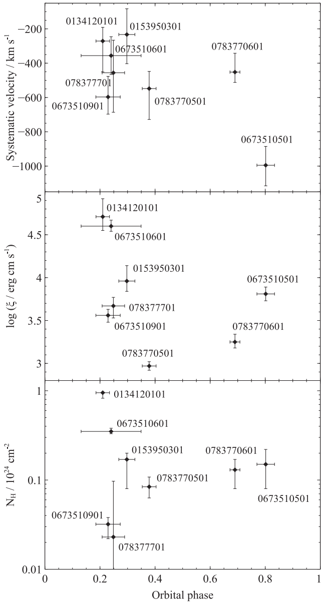
Figure 10. Top plot: Systematic velocity of the ionized absorber with respect to the orbital phase during each observation. Middle plot: Ionization parameter of the absorber versus the orbital phase during each observation. Bottom plot: Column density of the absorber versus the orbital phase during each observation.
