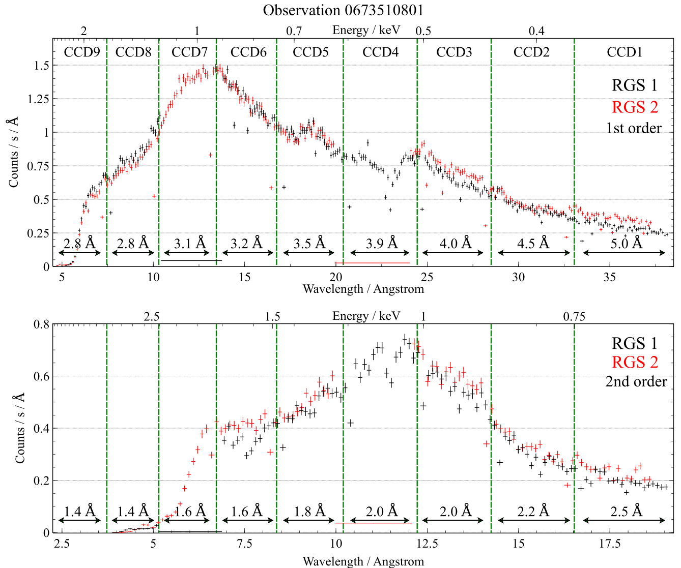
Figure A1. The average count rate per Å in the first and the second order of both RGS 1 and 2 instruments during the highest count rate observation 0673510801. The top plot contains the first-order count rates and the bottom plot contains the second-order count rates. RGS 1 data are in black, while RGS 2 data are red. Green vertical dashed lines show the approximate positions of chip gaps and the labels list the approximate chip sizes in Å. CCD numbers are listed on the top of the figure. The count rate per CCD can be approximated as the sum of the count rates per Å times the CCD width (in Å) of both orders.
