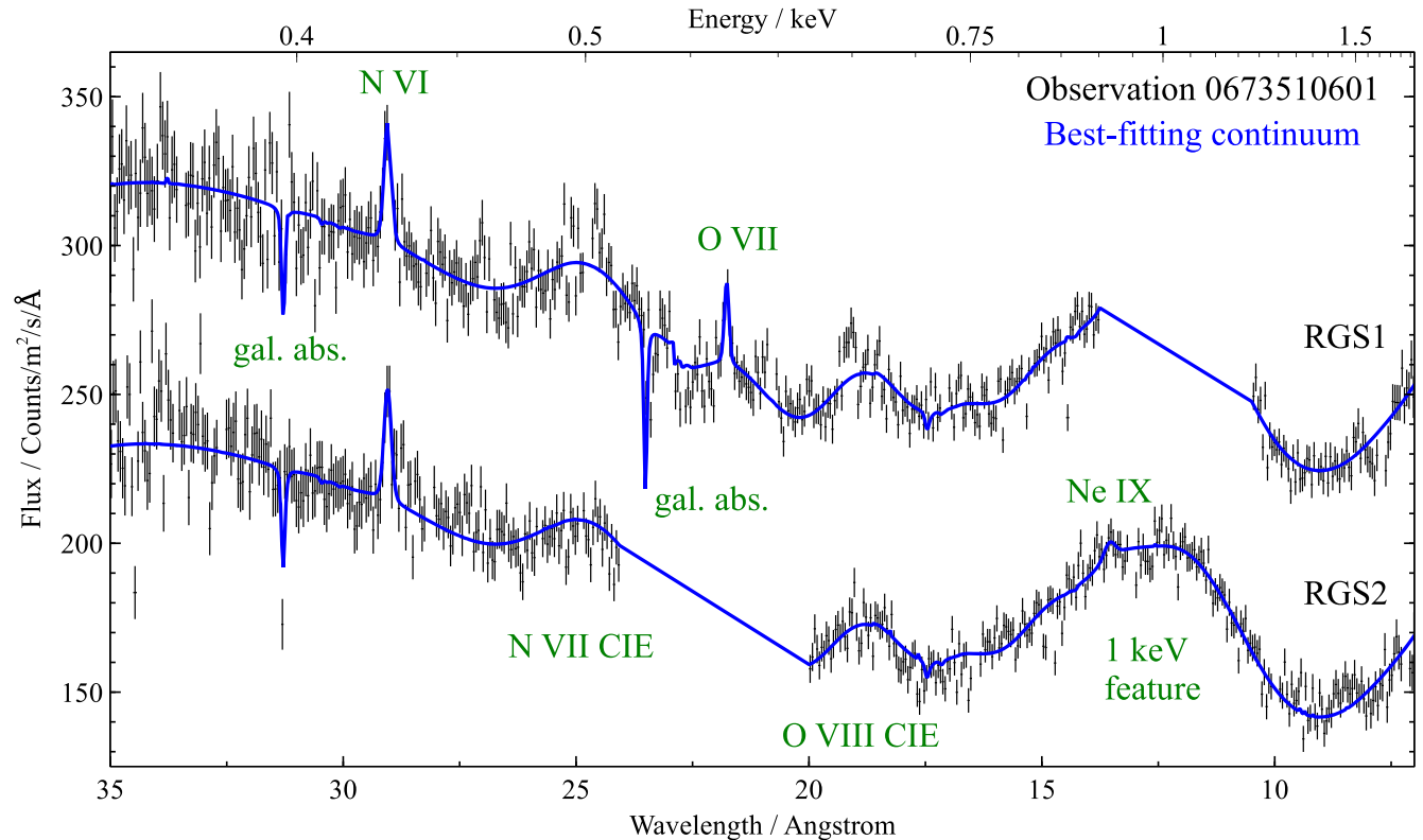
Figure 2. Example 35 Å (0.35 keV) to 7 Å (1.8 keV) spectrum of Her X-1 using RGS 1 and RGS 2 (Obs ID 0673510601). RGS1 data are shifted by a constant amount for plotting purposes and data from both detectors are heavily overbinned for clarity. Individual spectral components are named with green labels. Data between 11 and 14 Å in RGS 1 and between 20 and 24 Å in RGS 2 are missing because of chip gaps.
