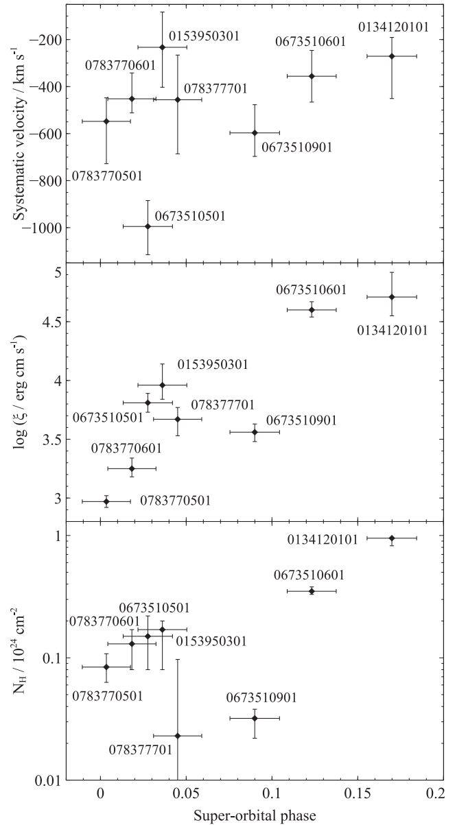
Figure 11. Top plot: Systematic velocity of the ionized absorber with respect to the superorbital phase during each observation. Middle plot: Ionization parameter of the absorber versus the superorbital phase during each observation. Bottom plot: Column density of the absorber versus the superorbital phase during each observation.
