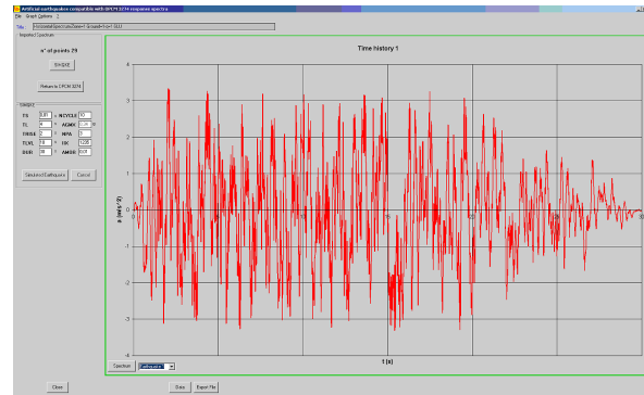
Fig. 7 Acceleration ( \text{m/sec}^2 ) vs. time (sec) – vertical time history 3.
