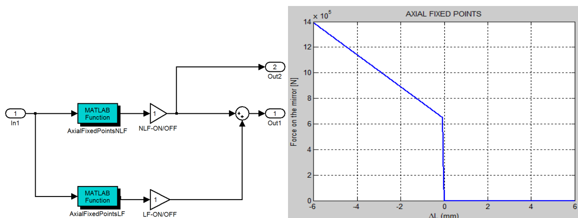
Fig. 6 Axial Fixed Points block insight (left) and nonlinear force-displacement curve (right)
