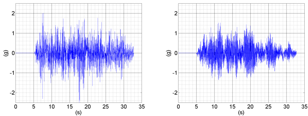
Fig. 9 Mirror acceleration along y axis: telescope pointing to horizon ( left ) and zenith ( right )
