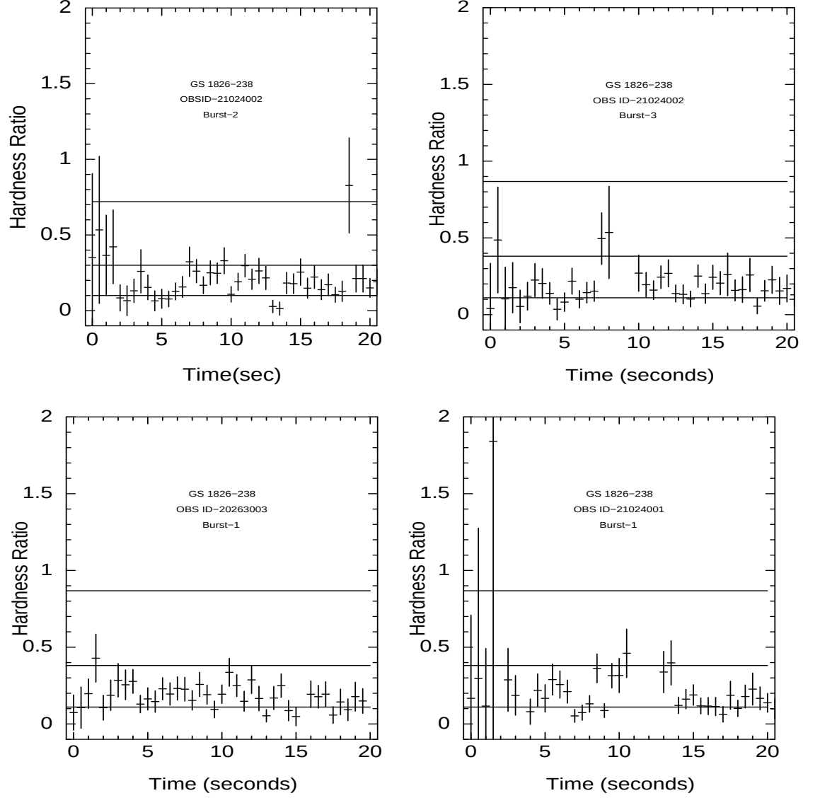
Figure 2: Hardness Ratio between two energy bands (1.8-10) keV and (15.0-30.) keV near the peak of bursts, obtained using background subtracted lightcurves from two instruments MECS and PDS . For details about background subtraction see text. The three horizontal lines starting from bottom in each plot represents ratios at 2.0 keV, 2.5 keV and 3.0 keV respectively.
