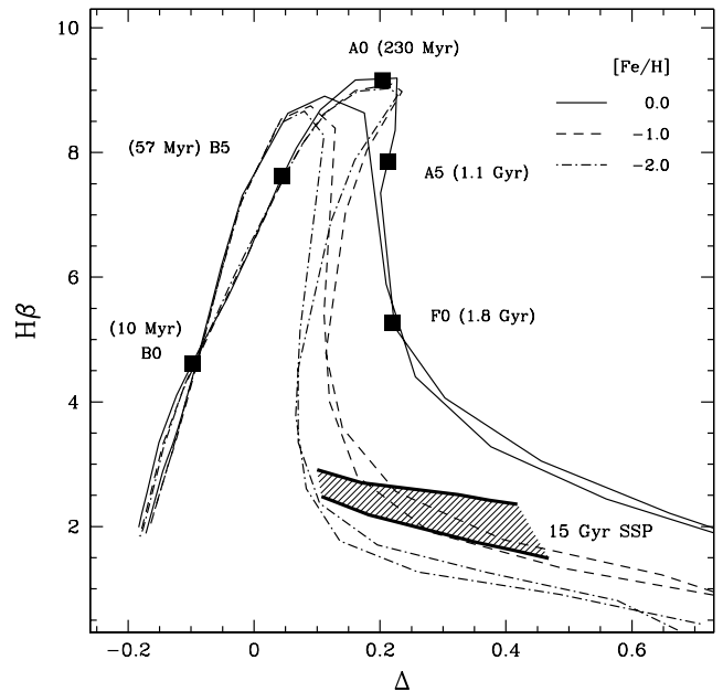
FIG. 7.—Theoretical diagram for the H\beta Lick index (in Å) vs. the Balmer jump \Delta index (in magnitude scale). Thin curves are the expected locus for MK V stars of different temperatures, from 5000 to 50,000 K, surface gravity ( \log g = 4 and 5, the latter being the shelf of curves peaking at slightly higher values of H\beta ), and metallicity (from [\text{Fe}/\text{H}] = -2 to solar, as labeled). Theoretical indices rely on the BLUERED library of synthetic stellar spectra (Bertone 2001; Bertone et al. 2003). The empirical spectral type vs. effective temperature calibration of Johnson (1966) is marked on the (\log g, [\text{Fe}/\text{H}]) = (5, 0.0) curve, together with the estimated MS lifetime of stars, as derived from Buzzoni (2002). The hatched area is the region for the 15 Gyr SSP models of Buzzoni (1989), with a different HB morphology. The lower edge of the area is for a red-clump HB morphology, while the upper edge is for a blue HB. SSP metallicity spans the range [\text{Fe}/\text{H}] = -2.27 to +0.22 dex, in the sense of increasing \Delta .
