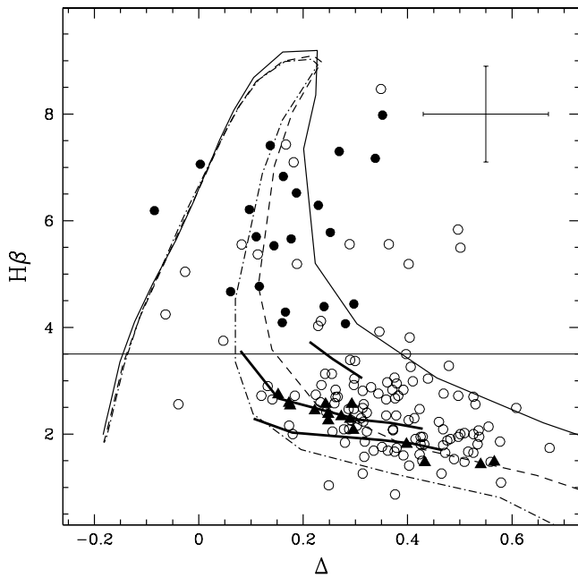
FIG. 8.—M31 GC distribution in the H\beta vs. \Delta index plane. Reference curves for \log g = 5 stars of different temperature (from 5000 to 50,000 K) and metallicity ( [Fe/H] from -2 to solar) are reported from Fig. 7. Sample A (i.e., color-selected) BLCCs are singled out (filled circles). By definition, sample B comprises all the targets in the plot above the H\beta = 3.5 Å threshold, as marked (40 objects with available indices from Table 1). For comparison, triangles show the Brodie & Huchra (1990) data for MW GCs, while thick solid lines are the locus for the Buzzoni (1989) SSP models with t = 15, 8 , and 2 Gyr (in the sense of increasing H\beta ), red HB morphology, and metallicity [Fe/H] = -2.27 to +0.22 . Typical error bars for M31 data are shown at the top right.
