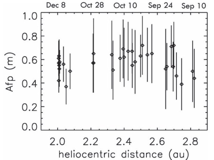
Figure 2. Coma photometry of 2I/Borisov according to the CARA network. The Afp values have been normalized to a phase of 30^\circ .
