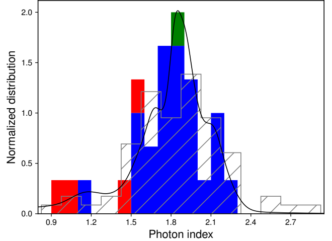
Fig. 5. Distribution of the power-law photon index in our sample as obtained from the baseline model, phabs × zpowerlw . The colour code is as follows: green for the radio-loud object, red for the marginal detections, blue for all the other sources. The same convention will be used, when relevant, in all of the following figures. The solid line represents an approximated probability density function that also takes into account the uncertainty in each measurement of \Gamma (see the text for more details). The dotted histogram is the (normalized) distribution of hard X-ray continuum slopes for the quasars in the CAIXA sample, corrected for a luminosity-dependent reflection component (Bianchi et al. 2009).
