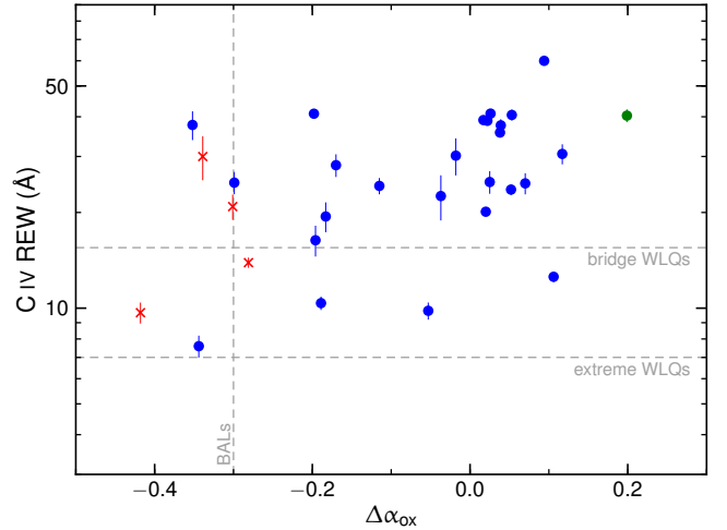
Fig. 10. Rest equivalent width of the C IV \lambda 1549 Å emission line, as obtained from our custom fits of the SDSS spectra, plotted against \Delta\alpha_{\text{ox}} . There is a hint of a possible correlation, confirmed at the 98.5% significance by the Pearson’s \rho and Kendall’s \tau tests. For reference, we also show the typical thresholds for two quasar populations known to exhibit enhanced rates of X-ray weakness, that is, BAL ( \Delta\alpha_{\text{ox}} < -0.3 ; Liu et al. 2018) and weak-line (extreme subset: C IV REW < 7 Å; bridge subset: C IV REW = 7\text{--}15.5 Å; Ni et al. 2018) quasars.
