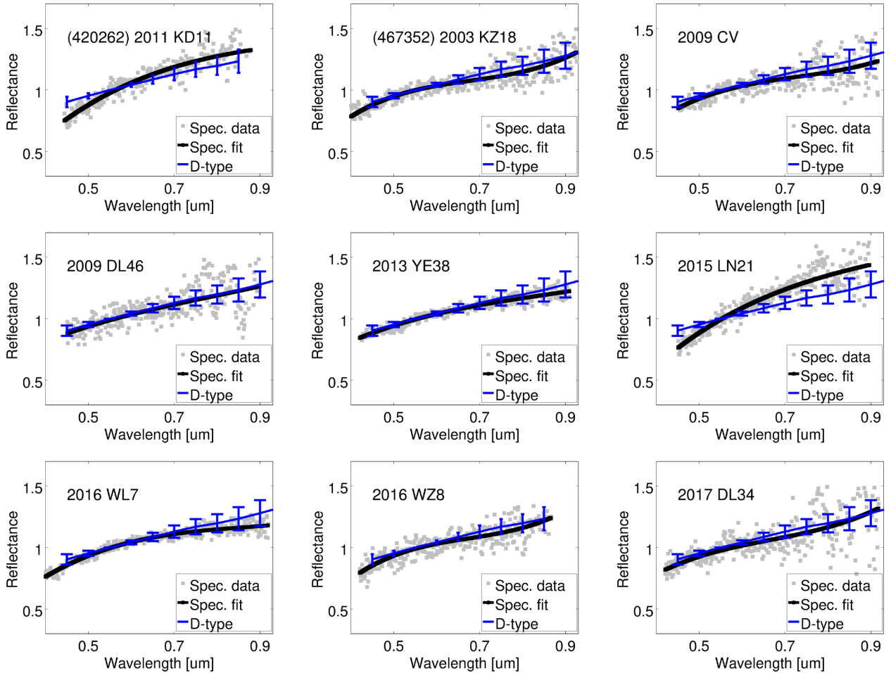
Figure 2. Visible spectra of (420262) 2011 KD11, (467352) 2003 KZ18, 2009 CV, 2009 DL46, 2013 YE38, 2015 LN21, 2016 WL7, 2016 WZ8, and 2017 DL34 are shown in grey. All spectra are normalized to 0.55 \mu\text{m} . A splinefit function (piecewise third-order polynomial fit) of the data is shown in black. The D taxonomic mean spectrum and its standard deviation defined by DeMeo et al. (2009) are shown in blue for comparison.
