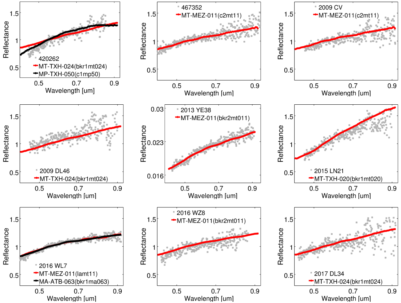
Figure 3. Plot of the asteroid spectra versus the best matched spectrum of carbonaceous chondrites from RELAB data base. The asteroid is identified by its designation and is plotted in grey, the RELAB spectrum corresponding to Tagish Lake is shown in red and it is referenced by its sample ID and file name. For the two cases where the best match was a different meteorite we plot their spectrum in black. See Table 3 for additional details. All spectra are normalized to 1 at 0.55 \mu\text{m} .
