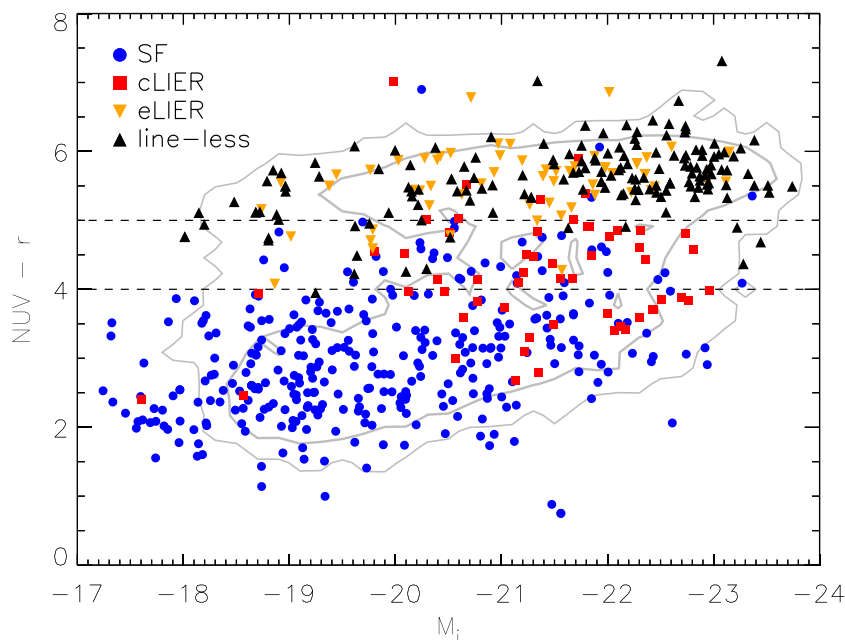
Figure 3. MaNGA galaxies in the NUV - r versus M_i (colour-magnitude) diagram. Galaxies are divided according to the emission-line-based classification introduced in Paper I (see also Section 2 of this work). Contours represent galaxy density in the MaNGA parent sample, while dashed lines provide a simple division between the red sequence ( NUV - r > 5 ), green valley ( 4 < NUV - r < 5 ) and blue cloud ( NUV - r < 4 ). The green valley is preferentially occupied by cLIER galaxies, while eLIER and line-less galaxies are mostly found on the red sequence ( NUV - r > 5 ).
