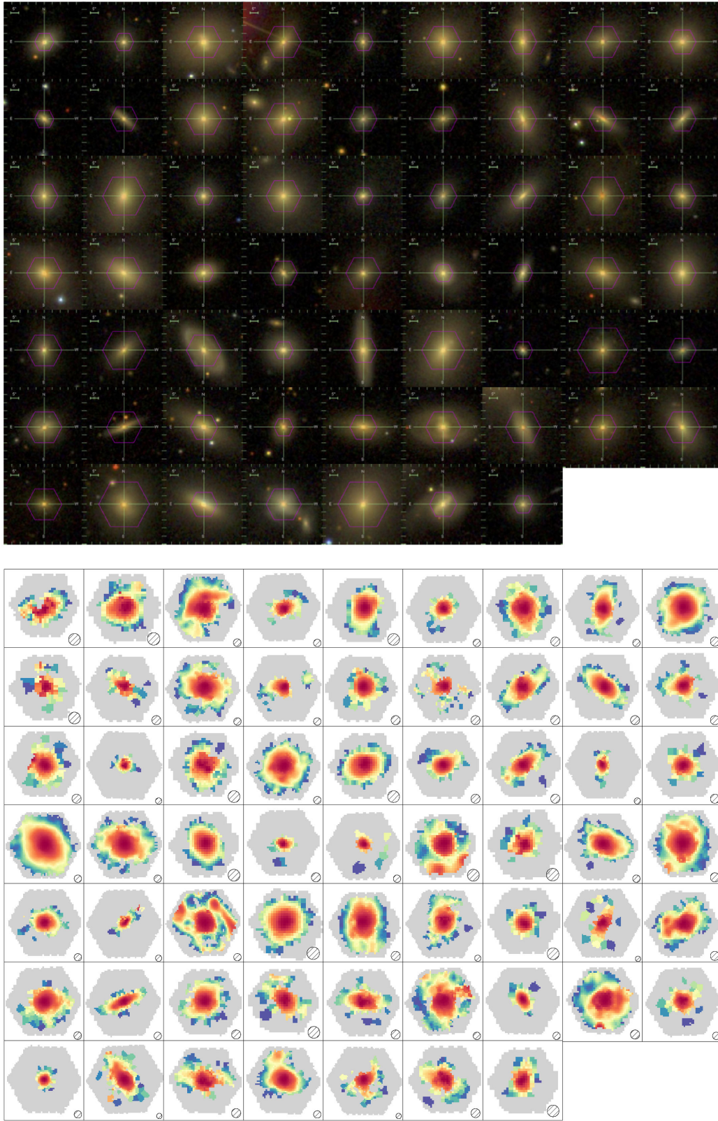
Figure B2. Top: SDSS g-r-i colour composite images (with MaNGA IFU bundle FoV superimposed) for the sample of eLIER galaxies studied in this work. Bottom: MaNGA H\alpha flux maps for the sample of eLIER galaxies studied in this work.
