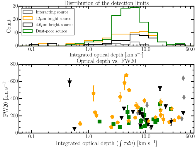
Fig. 6. Full-width at 20% of the intensity (FW20) vs. the integrated optical depth of the H I lines ( \int \tau dv ). Symbols follow the WISE colour-colour classification shown in Fig. 1. The histogram in the top panel shows the distribution of the 3\sigma detection limit in optical depth for the non-detections of the each subsample.
