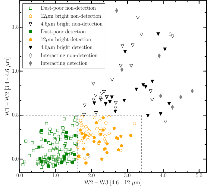
Fig. 1. WISE colour-colour plot for the sources of the sample, separated into H I detections (filled symbols) and H I non-detections (empty symbols). Dust-poor galaxies are green squares, 12 \mu\text{m} bright sources are orange pentagons and 4.6 \mu\text{m} bright sources are black triangles. Interacting sources are grey diamonds. The dashed lines indicate the cut-offs of the WISE colours we used to classify our sources. Further details on the classification of the sources are shown in Table 1.
