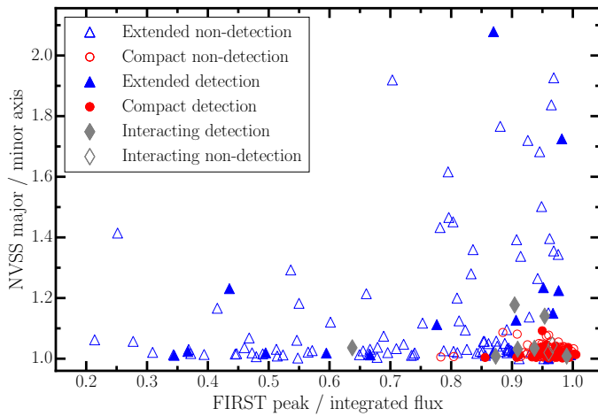
Fig. 2. Radio morphological classification of the sample. Red circles indicate compact sources, extended sources are indicated by blue triangles, interacting sources are shown in grey diamonds. H I detections are indicated by filled symbols, while empty symbols represent non-detections.
