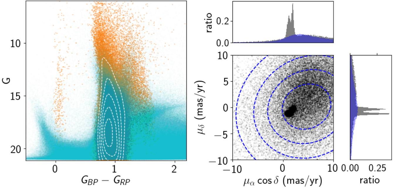
Fig. 3. Left: CMD of the GalMod theoretical population synthesis model (orange) overlayed on all Gaia DR2 sources (cyan) of the same area of the Magellanic Bridge. The white contour levels show the model number density distribution in steps of 20 000 sources starting at the centre. Right: proper motion distribution in right ascension and declination of Gaia DR2 sources (black). The contour levels of the foreground simulation are indicated with blue dashed lines and contain each 20 000 sources. The corresponding ratios between the two proper motion components for the Gaia DR2 proper motions are shown in grey and for the GalMod simulation in blue. The LMC and the SMC are visible as two narrow peaks, while the MW foreground stars are more spread out.
