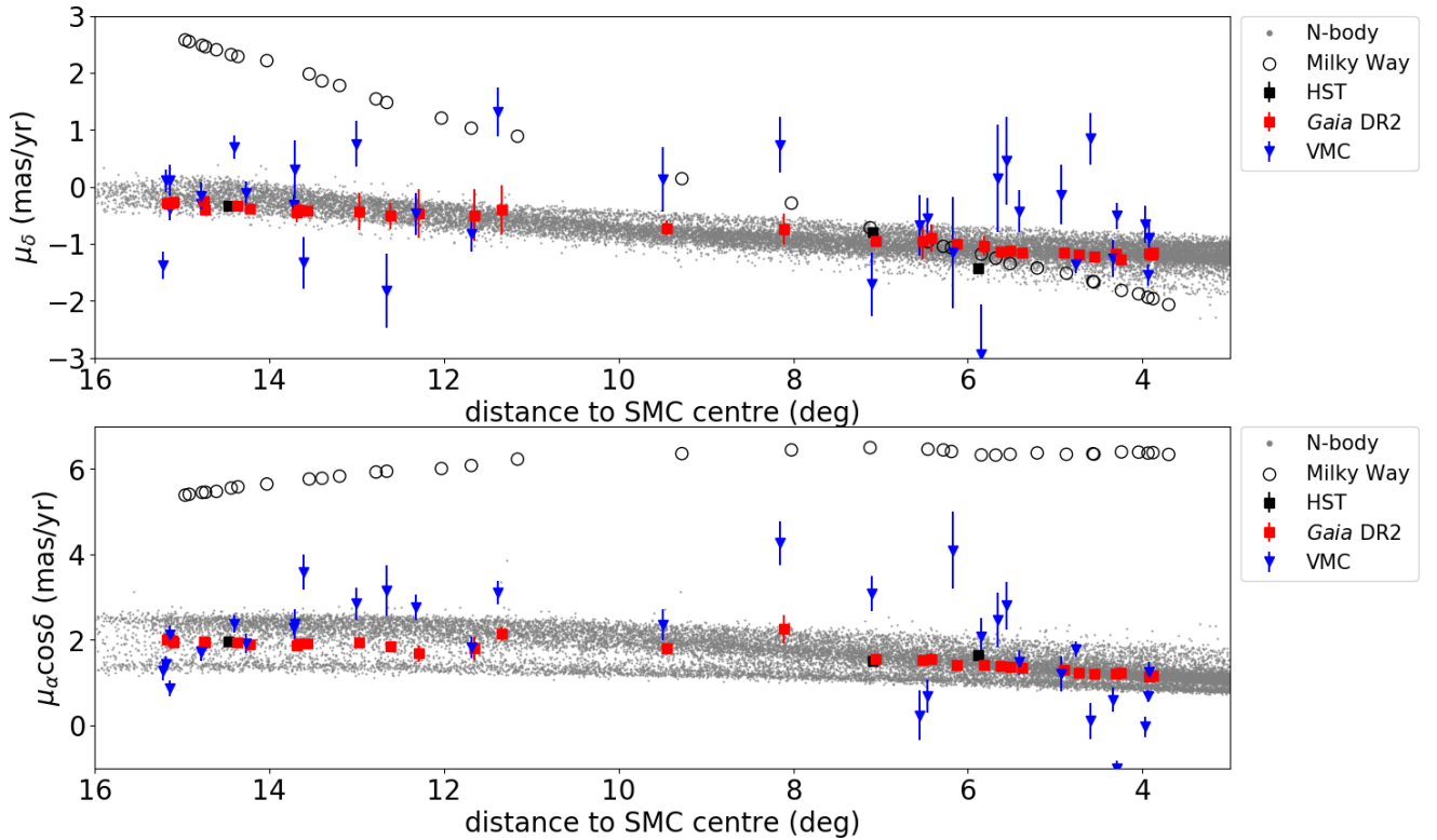
Fig. 11. Proper motions \mu_\delta and \mu_\alpha \cos \delta for the sample of stars selected based on StarHorse distances (>30 kpc). Proper motions of VMC (blue triangles), Gaia DR2 (red squares), N-body particles (grey dots), HST measurements (black squares) and the GalMod Milky Way foreground (empty circles) are shown as a function of projected distance from the SMC centre.
