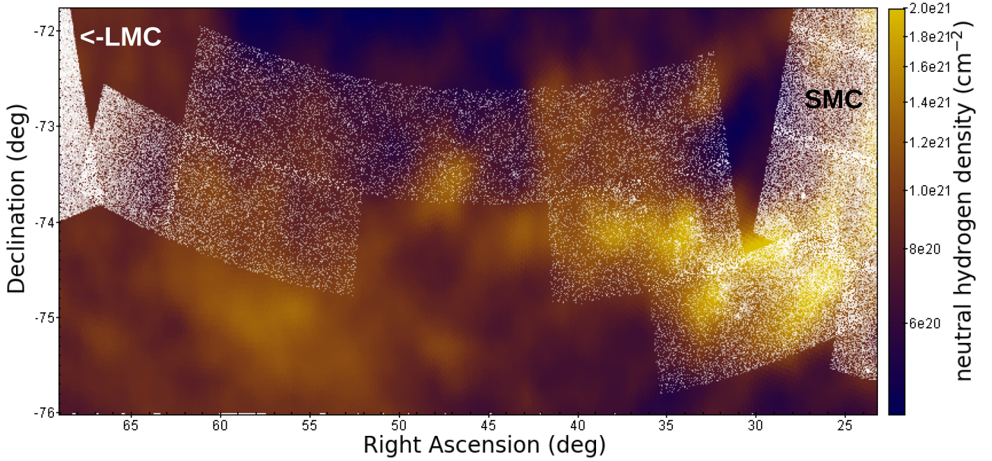
Fig. 1. Distribution of Magellanic Bridge stars from the VMC- Gaia DR2 sample (white) superimposed on the distribution of H I gas (HI4PI Collaboration 2016). The rectangular structures represent the shape of the VMC tiles.
