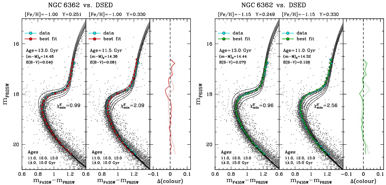
Figure 13. Same as Figure 10, but for NGC 6362.
