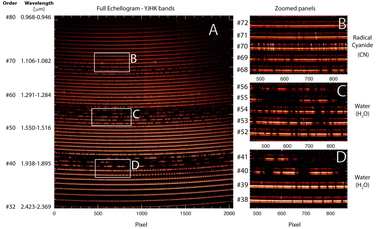
Figure 2. Panel A: GIANO echellogram of comet Lovejoy acquired on UT 2015 February 2. The panel shows the full echellogram covering 50 orders. Pixel column number (x-axis) and order number and wavelength range (y-axis) are labeled. The order number increases from the bottom (#32) to the top (#80). Wavelength decreases from left to right within each order, and decreases from bottom to top across the echellogram. Each order contains a group of four arc-shaped tracks. The upper two tracks (3, 4) of each group correspond to image slices of fiber B and the lower two tracks (1, 2) to fiber A (slices); in this frame the photometric nucleus of comet was centered on fiber A, where strong cometary continuum is seen in all orders. Absorption features of terrestrial atmospheric gases appear throughout the echellogram (e.g., at the top and bottom of H band), along with many sky emission lines of OH (Meinel bands) that fill the fibers uniformly so are equally bright in tracks 1, 2, 3, and 4. We outline regions in which we detected cometary water and radical CN. Cometary H 2 O lines are brighter near the nucleus (tracks 1 and 2) but also appear in the off-nucleus position (3 and 4). The lines of radical CN (a product species) are equally bright in tracks 1, 2, 3, and 4. Zoomed panels B-D: pixel column and order numbers are shown on the x- and y-axis, respectively. Panel B shows zoomed box B from panel A (near 1.1 μm) in which radical CN and probably water are detected. Panels C and D show the water vibrational bands near 1.4 and 2 μm detected in boxes C and D (panel A).
