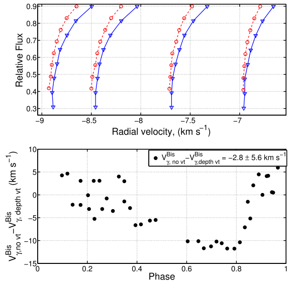
Figure 8. Top panel: comparison of synthetic bisectors computed with the depth-dependent microturbulent velocity model (triangles) and constant microturbulent velocity v_{\text{mic}} = 2 \text{ km s}^{-1} (circles). Bottom panel: difference between the gamma velocities of RR Lyr derived with different sets of bisector grids: with ( V_{\gamma}^{\text{Bis, depth-dep. } v_{\text{mic}}} ) and without depth-dependent v_{\text{mic}} stellar-atmosphere models ( V_{\gamma, \text{RR Lyr}}^{\text{Bis, constant } v_{\text{mic}}} ).
