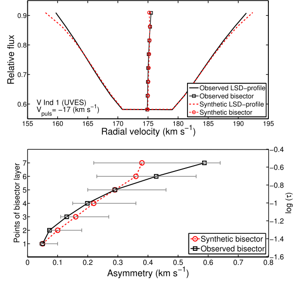
Figure 5. Comparison of observed (solid) and best-fitting theoretical (dashed) LSD profiles (top panel) and bisectors (bottom panel) for our first V Ind spectrum ( \phi = 0.19 ; see Table 3). The best fit corresponds to v_{\text{puls}} = -17 \pm 1 \text{ km s}^{-1} . The grey error bars in the bottom panel correspond to the estimated errors in the method for determining v_{\text{puls}} , i.e. 1 \text{ km s}^{-1} . The optical depth scale on the right ordinate axis was computed from synthetic spectra built with the atmospheric parameters derived in Paper I: T_{\text{eff}} = 7000 \text{ K} , \log g = 2.3 \text{ dex} , v_{\text{mic}} = 1.6 \text{ km s}^{-1} and [\text{Fe}/\text{H}] = -1.3 \text{ dex} . The divergence between the observed and theoretical bisectors in layer 7 is caused by the lower S/N ratio of the LSD profile in this layer (see text for details). While the model bisector does not follow the shape of the observed ones exactly, the two agree reasonably well within the uncertainties.
