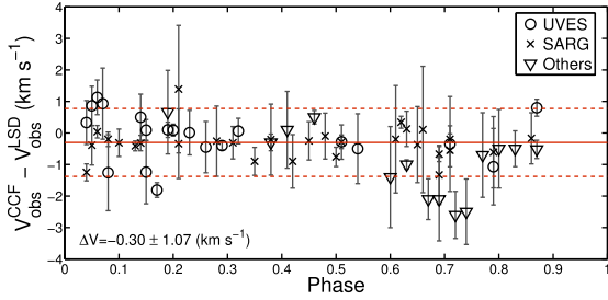
Figure 3. Differences between radial velocity estimates derived with the cross-correlation method, v_{\text{obs}}^{\text{cor}} , and with the LSD profile method, v_{\text{obs}}^{\text{LSD}} . Observations from different spectrographs are labelled respectively.
