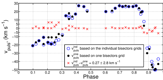
Figure 7. Difference between pulsational velocities for each spectrum of RR Lyr derived with individual sets of bisector grids and one bisector grid, number 087, for all observed spectra.
