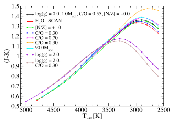
Figure 11. ( J − K ) as a function of the effective temperature for COMARCS models with solar metallicity. The standard parameters are \log(g \text{ [cm s}^{-2}\text{]}) = 0.0 , M/M_{\odot} = 1.0 , solar abundances ( \text{C}/\text{O} = 0.55 , [\text{N}/\text{Z}] = 0.0 ) and usage of the BT2 line list for water below 4000 K (black). The result of changing C/O to 0.3 (blue), 0.7 (magenta) and 0.9 (orange), of increasing nitrogen by a factor of 10 ( [\text{N}/\text{Z}] = +1.0 , green) or the mass to 90 M_{\odot} (cyan) is shown. In addition, we demonstrate the effect of taking the \text{H}_2\text{O} opacities from the SCAN data (red) and of adopting \log(g \text{ [cm s}^{-2}\text{]}) = 2.0 with C/O = 0.55 (violet) or 0.3 (brown).
