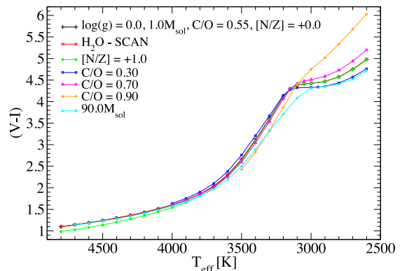
Figure 10. ( V − I ) as a function of the effective temperature for COMARCS models with solar metallicity and \log(g \text{ [cm s}^{-2}\text{]}) = 0.0 . Parameters, symbols and lines are like in Fig. 9.
