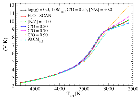
Figure 9. ( V − K ) as a function of the effective temperature for COMARCS models with solar metallicity and \log(g \text{ [cm s}^{-2}\text{]}) = 0.0 . The standard parameters are M/M_{\odot} = 1.0 , solar abundances ( \text{C}/\text{O} = 0.55 , [\text{N}/\text{Z}] = 0.0 ) and usage of the BT2 line list for water below 4000 K (black). The result of changing C/O to 0.3 (blue), 0.7 (magenta) and 0.9 (orange), of increasing nitrogen by a factor of 10 ( [\text{N}/\text{Z}] = +1.0 , green) or the mass to 90 M_{\odot} (cyan) is shown. In addition, we demonstrate the effect of taking the \text{H}_2\text{O} opacities from the SCAN data (red).
