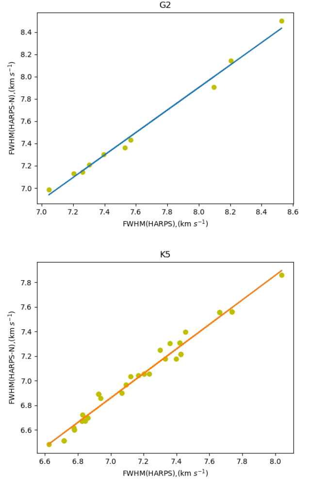
Fig. 5. Calibration of FWHM examples in order to derive v \sin i for common stars sampled in HARPS and HARPS-N data.
