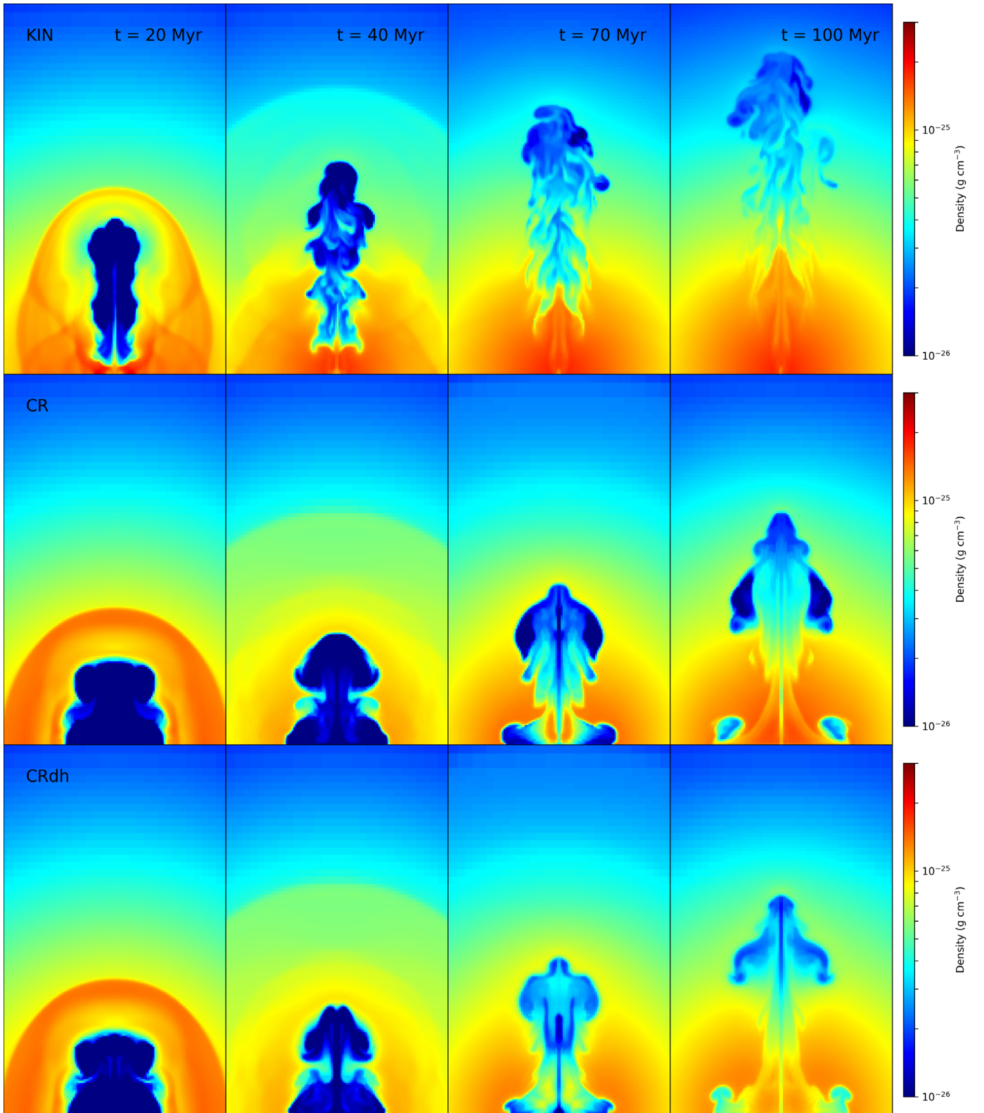
Figure 1. Evolution of the gas density for simulations of kinetic-energy-dominated jets (KIN; top row), CR-dominated jets with no diffusion or heating (CR; middle row), and CR-dominated jets with diffusion and collisional heating (CRdh; bottom row). The physical scale for each panel is 60 kpc by 100 kpc.
