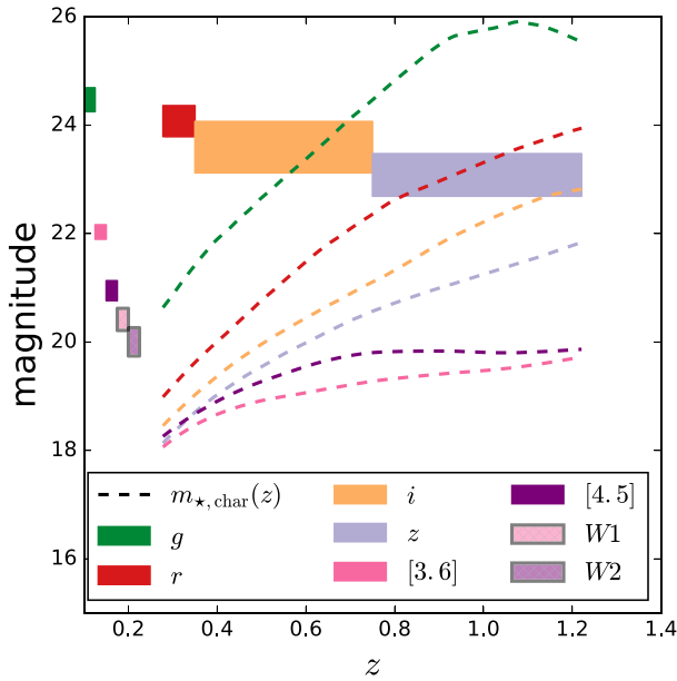
Figure 2. A comparison of photometric depths (bars of constant magnitude) and the redshift variation of the characteristic magnitude m_{*,\text{char}}(z) (dashed lines) over the relevant redshift range. The median and the 1\sigma variation of the 50 percent completeness for the DES griz bands are shown with green, red, orange, and purple bars, respectively. The 10\sigma depth of [3.6] and W1 ([4.5] and W2) are shown in pink (dark purple), where the WISE passbands are marked with black boundaries. The redshift ranges of the riz bands stand for the redshift ranges over which we use those bands to apply the magnitude cut (see Section 3.3.2), while the limits in the other bands (i.e. g [3.6][4.5]W1W2) all appear on the left.
