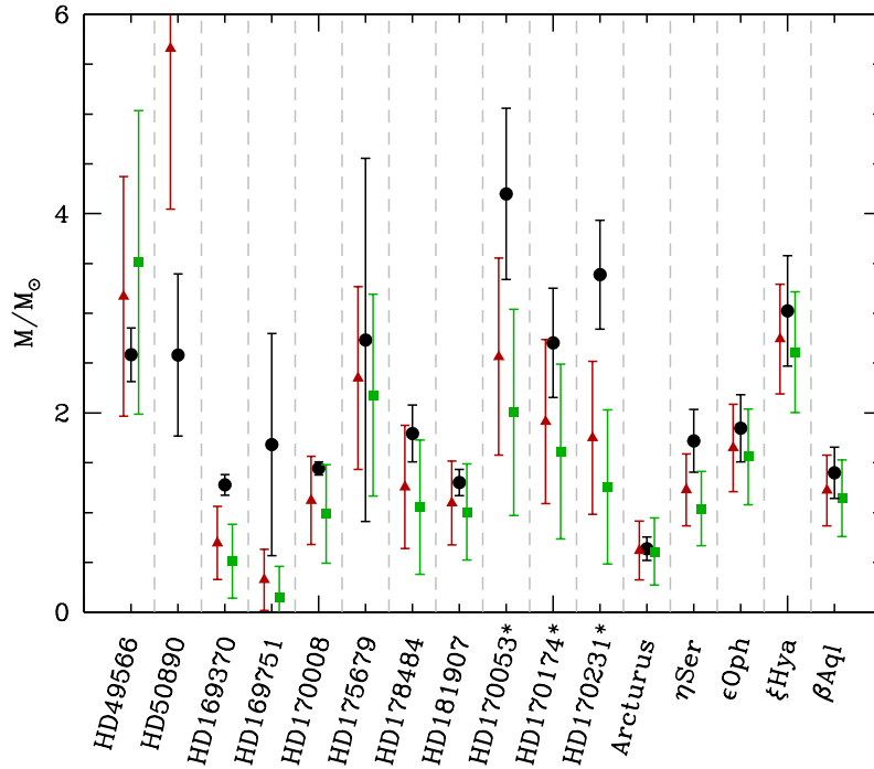
Fig. 2. Comparison between the masses obtained by different combinations of the observational constraints available. Masses are determined using asteroseismic constraints ( \nu_{\max} , \Delta\nu ) and T_{\text{eff}} (black dots); using \nu_{\max} , T_{\text{eff}} , the extinction from Drimmel's model, and the stellar radius from the HIPPARCOS parallax (using T_{\text{eff}} , red triangles); and using \Delta\nu and the stellar radius from the HIPPARCOS parallax (using T_{\text{eff}} ) and stellar extinction by Drimmel's model (green squares). Asterisks indicate stars that are members of NGC 6633.
