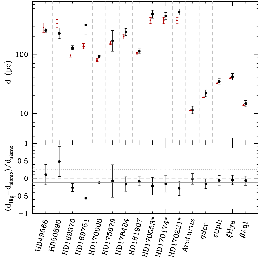
Fig. 3. Comparison between the distances determined from asteroseismic constraints ( \nu_{\max} , \Delta\nu ) and T_{\text{eff}} (black dots), and the HIPPARCOS distance (red triangles). In the lower panel, the grey solid line represents the weighted average difference, while the grey dashed lines represent a difference of 25%. Asterisks identify the cluster members.
