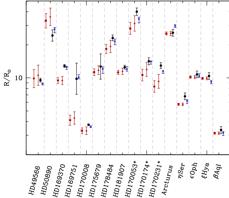
Fig. 1. Comparison between the radii obtained by different combinations of the available observational constraints. Radii are determined using asteroseismic constraints ( \nu_{\max} , \Delta\nu ) and T_{\text{eff}} (black dots); determined with PARAM (blue crosses); and using the parallax from the HIPPARCOS catalogue (van Leeuwen 2007), apparent magnitudes, and extinction from different prescriptions (red symbols). Squares represent radii computed with no extinction ( A_V = 0 ), and triangles extinctions from the 3D Galactic extinction model by Drimmel et al. (2003). Asterisks indicate stars that are members of NGC 6633.
