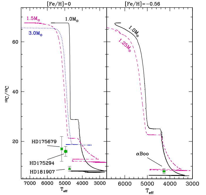
Fig. 12. ^{12}\text{C}/^{13}\text{C} data in our red giant stars that are segregated according to their metallicity (left and right panels include respectively sample stars with metallicity close to solar and [\text{Fe}/\text{H}] = -0.56 ). Same symbols as in Fig. 11. Theoretical ^{12}\text{C}/^{13}\text{C} surface abundance is shown from the ZAMS up to the TP-AGB. Various lines correspond to predictions of stellar models of different masses including effects of rotation-induced mixing (with an initial V_{\text{ZAMS}}/V_{\text{crit}} = 0.30 ) and thermohaline instability.
