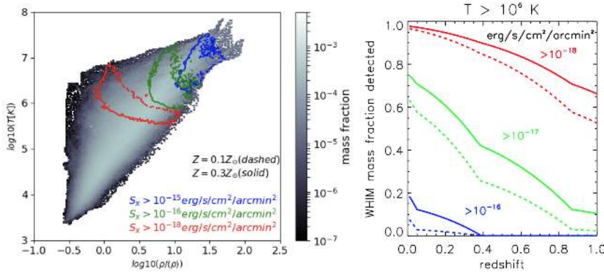
Fig. 4 (Left) Phase diagram of the gas in a comoving 85 Mpc 3 volume, simulated using 1024 3 cells with the ENZO code (Bryan et al., 2014) and including the effect of magnetic fields, radiative cooling, star formation, supermassive black holes, and of the thermal feedback from star-forming regions and AGN as detailed in Vazza et al. (2017). Lines indicate the sensitivity required to observe it. (Right) Distribution of the mass fraction of the gas at T > 10^6 K that is expected to be resolved, as a function of redshift, at different cuts in surface brightness in the 0.3–2 keV band, and for different metallicities.
