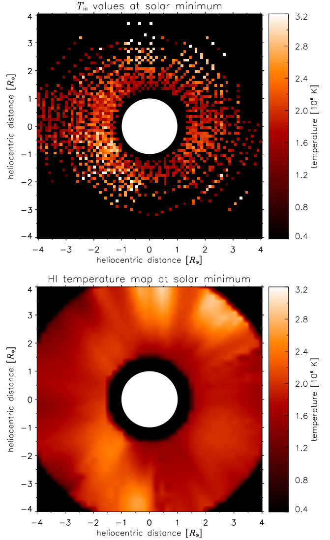
Fig. 6. Top panel: map of the T_{HI} values at solar minimum obtained by Dolei et al. (2016) from the analysis of the Ly \alpha line width. Bottom panel: adopted coronal HI temperature map.
