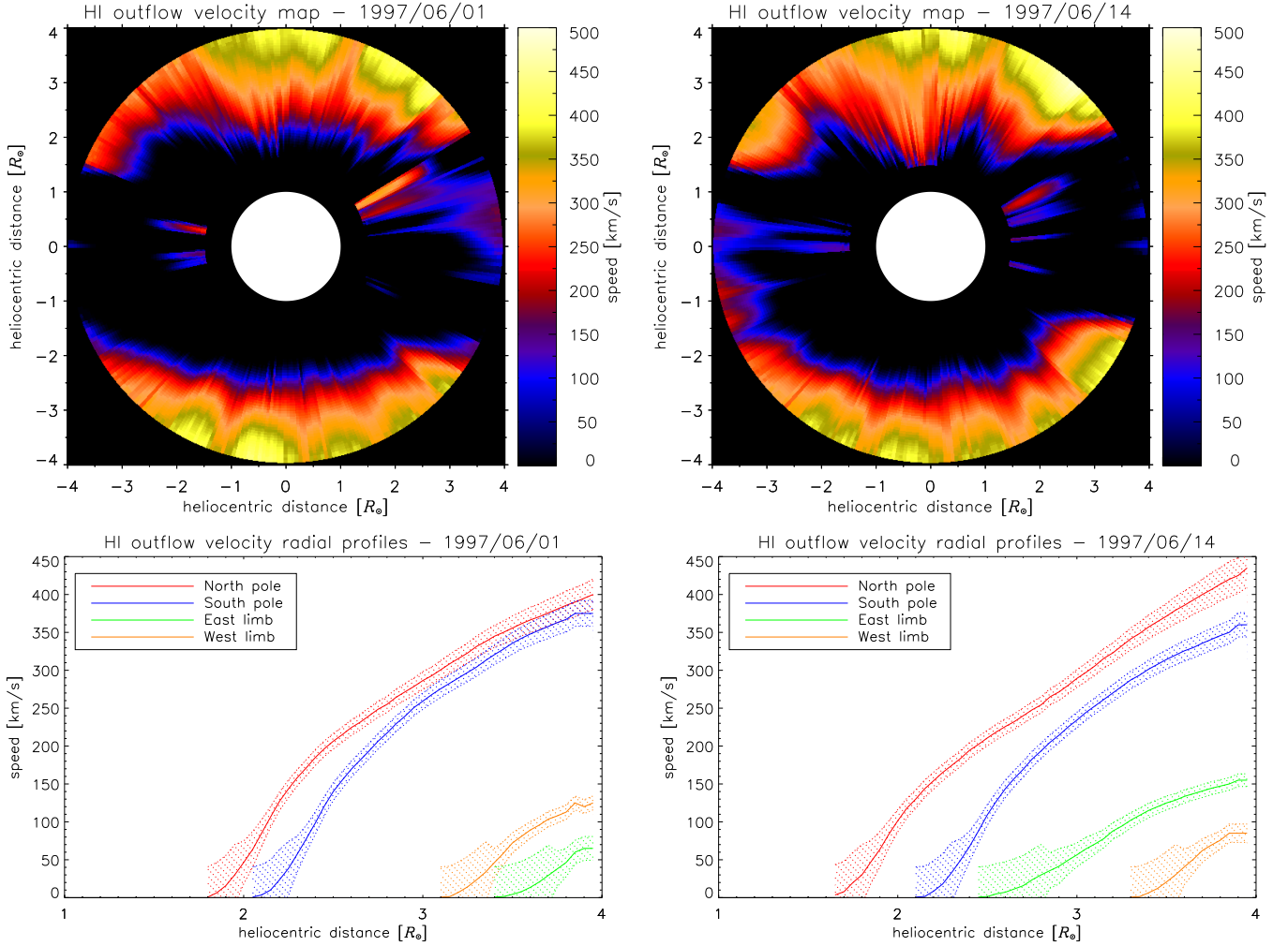
Fig. 7. Top panels: HI outflow velocity maps on the 1st (left) and 14th (right) June 1997. Bottom panels: HI outflow velocity radial profiles in the equatorial and polar regions on the 1st (left) and 14th (right) June 1997. The dotted areas represent the range of speed uncertainty as a result of an uncertainty of the reconstructed UV Ly \alpha line intensity by 3%, according to the variation rate of the effective Doppler dimming coefficient.
