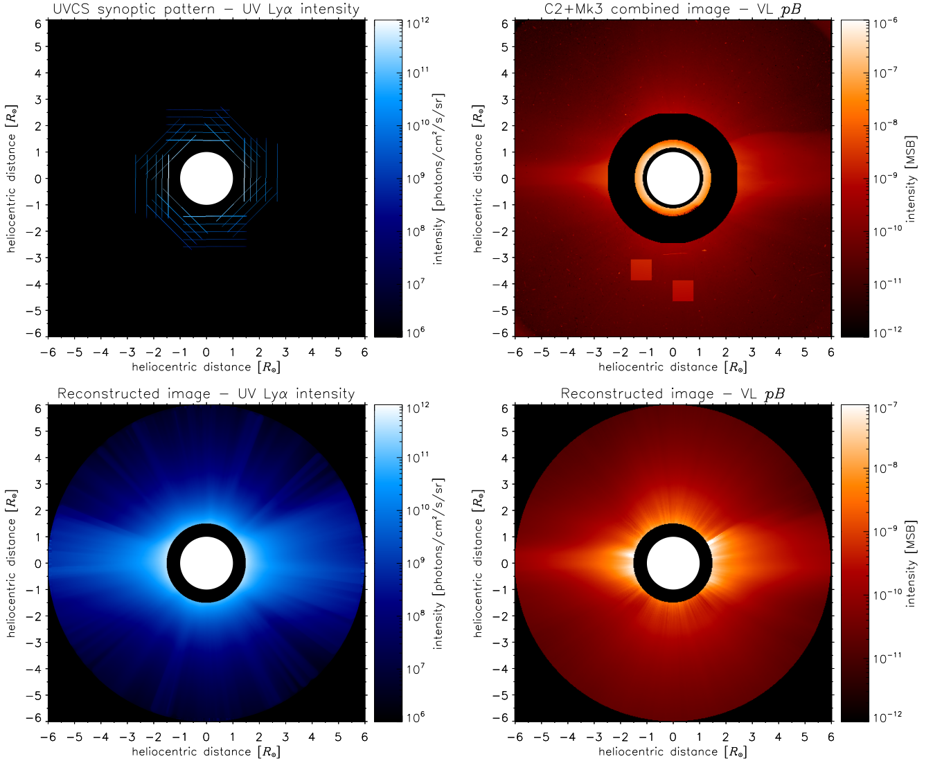
Fig. 2. Left panels: UV HI Ly \alpha line intensity on the 1st June 1997, in units of photons cm -2 s -1 sr -1 , as measured by the UVCS daily synoptic observation (top) and reconstructed between 1.5 and 6.0 R_\odot (bottom). Right panels: VL polarised brightness on the 1st June 1997, in units of Mean Solar Brightness (MSB), as measured by the LASCO C2 and Mk3 coronagraphs (top) and reconstructed between 1.5 and 6.0 R_\odot (bottom).
