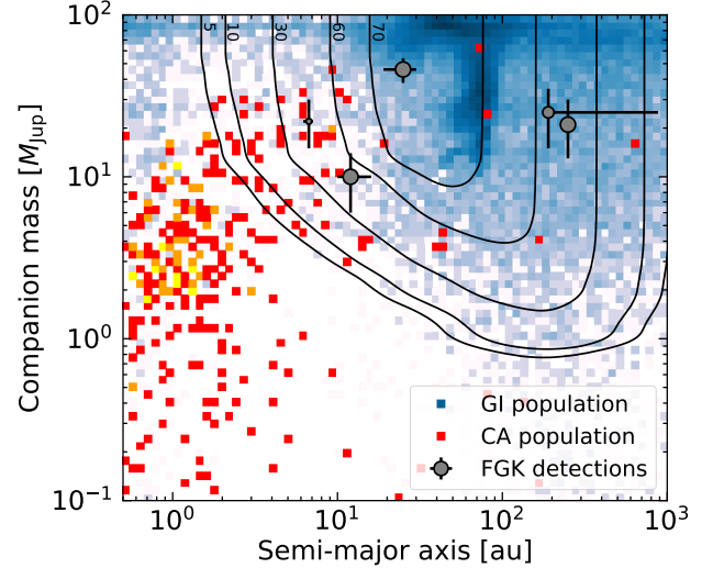
Fig. 4. Comparison of the depth of search of the SHINE survey for the 77 FGK stars in the sample with the population synthesis models based on the CA and GI formation scenarios presented in Sects. 3.2.1 and 3.2.2, respectively. The contour lines give the numbers of stars around which the survey is sensitive to substellar companions as a function of mass and semimajor axis. The CA companions are represented with shades of red (low density of companions) to yellow (high density of companions), and the GI companions are represented with shades of white (low density of companions) to blue (high density of companions). The apparent lower density of CA objects arises because the vast majority of the CA population is located outside the range of mass and semimajor axis considered in this plot. Only the detections around FGK stars are plotted.
