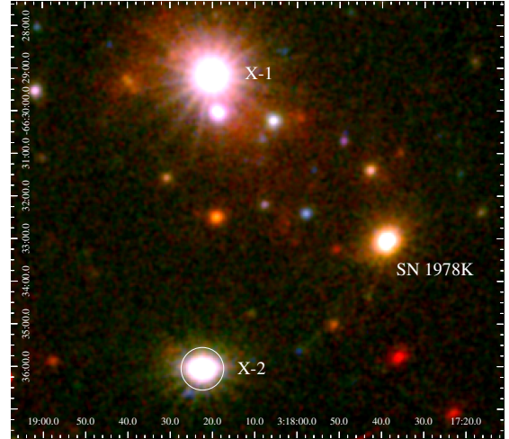
Fig. 1. XMM-Newton image of NGC 1313, which we obtained by combining all the data available from the 2017 EPIC-pn and MOS 1,2 observations. The 30''-radius circle around the ULX X-2 represents our default source extraction region. The red colour corresponds to 0.2–1 keV, green is for 1–2 keV, and blue is for 2–12 keV.
