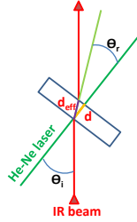
Figure 4: Schematic view of the geometry used for the measure of the effective sample thickness.
