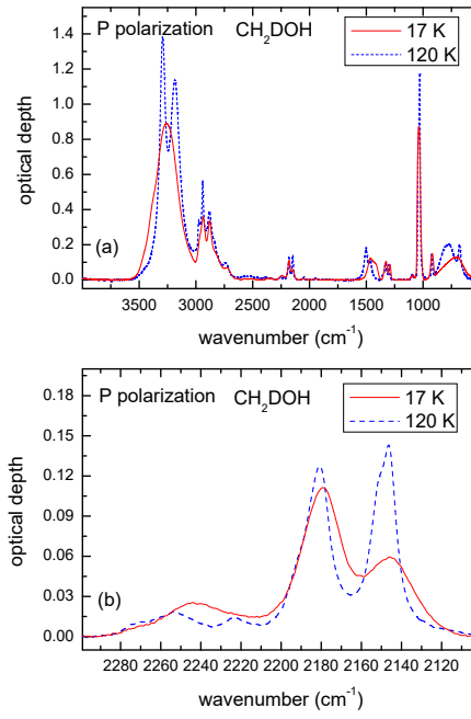
Figure 13: (a) CH 2 DOH spectra at 17 K and 120 K. (b) Detail of the CD stretching modes vibration region (2300-2100 cm -1 ). The sample is about 1 \mu m thick.
