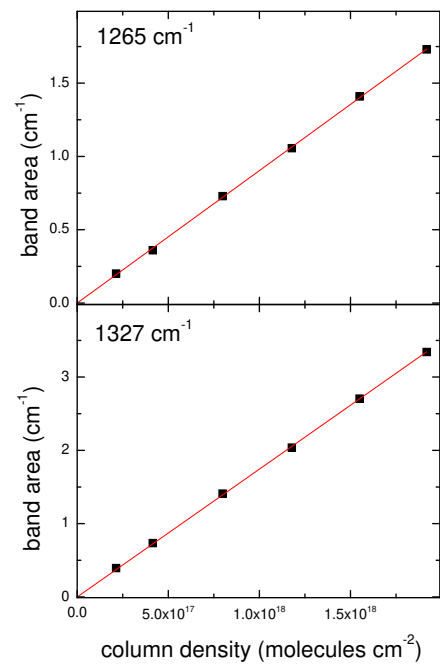
Figure 9: Measures of the P polarization band areas (1265 and 1327 cm -1 ) versus the column density for the CH 2 DOH deposited ice.
