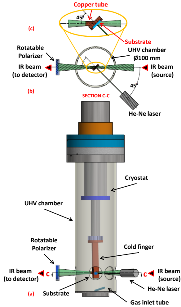
Figure 1: (a) Three-dimensional drawing of the UHV chamber system. (b) Top view section of the chamber. (c) Detail of the copper tube used to avoid gas deposition on the backside of the substrate (not to scale).
