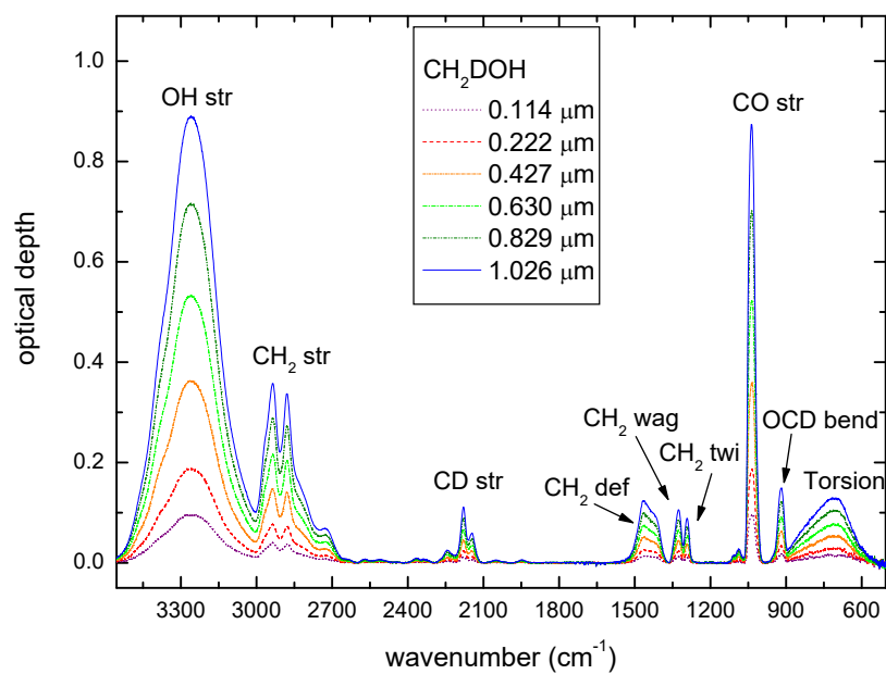
Figure 5: IR spectra of \text{CH}_2\text{DOH} ice acquired at various thicknesses in P polarization.
