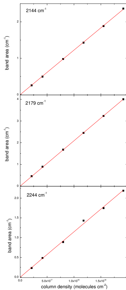
Figure 10: Measures of the P polarization band areas (2144, 2179 and 2244 cm -1 ) versus the column density for the CH 2 DOH ice.
