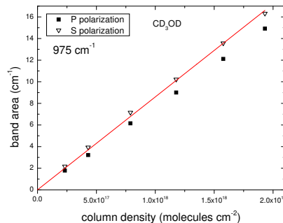
Figure 11: Measures of the CO stretching P and S polarization band areas versus the column density for the \text{CD}_3\text{OD} ice. The linear best fit is performed only on the S polarization data.
