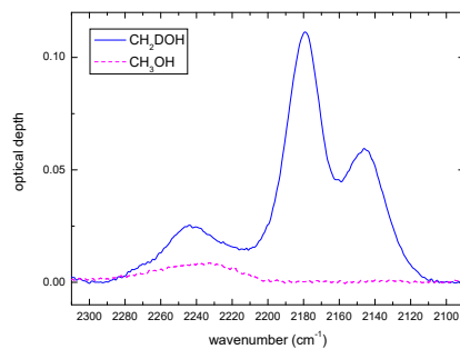
Figure 6: 2300-2100 \text{cm}^{-1} spectral region region for \text{CH}_3\text{OH} and \text{CH}_2\text{DOH} . The samples are about 1\text{ }\mu\text{m} thick.
