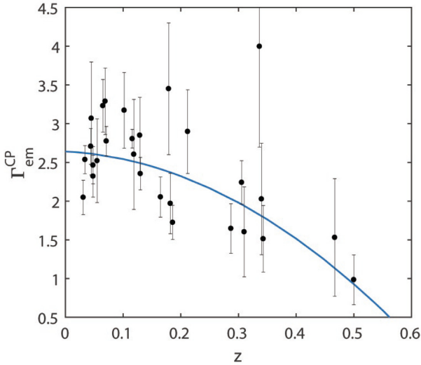
Figure 7. Same as Fig. 6, but with superimposed the best-fitting regression line with \chi^2_{\text{red,CP}} = 1.82 .
