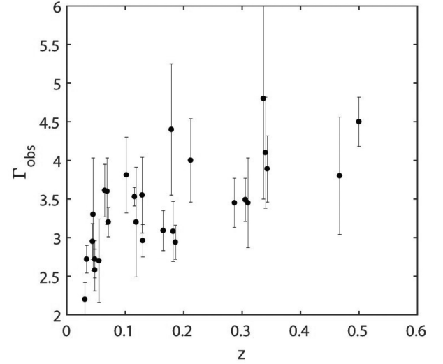
Figure 5. The values of \Gamma_{\text{obs}} with the corresponding error bars are plotted versus z for all blazars of S_0 .
