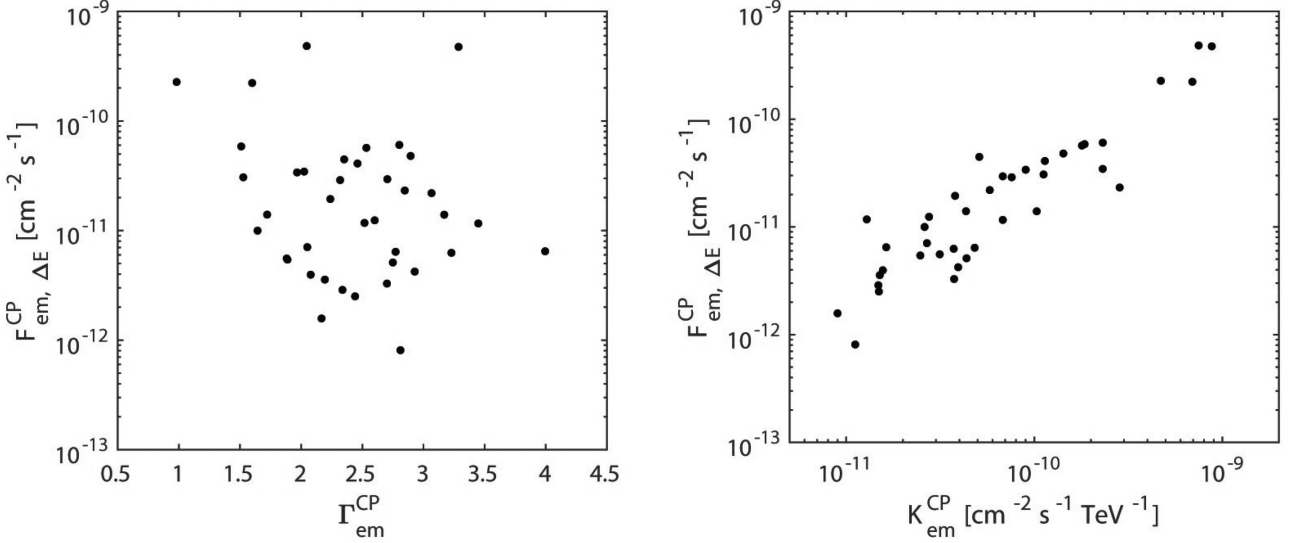
Figure 9. Left-hand panel: The values of F_{em, \Delta E}^{CP} are plotted versus \Gamma_{em}^{CP} for all blazars in \mathcal{S} . Right-hand panel: The values of F_{em, \Delta E}^{CP} are plotted versus K_{em}^{CP} for all blazars in \mathcal{S} .
