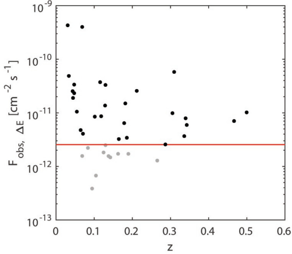
Figure 4. Out of the original sample S – represented by all points – we have constructed the subsample S_0 of sources denoted by black points.
