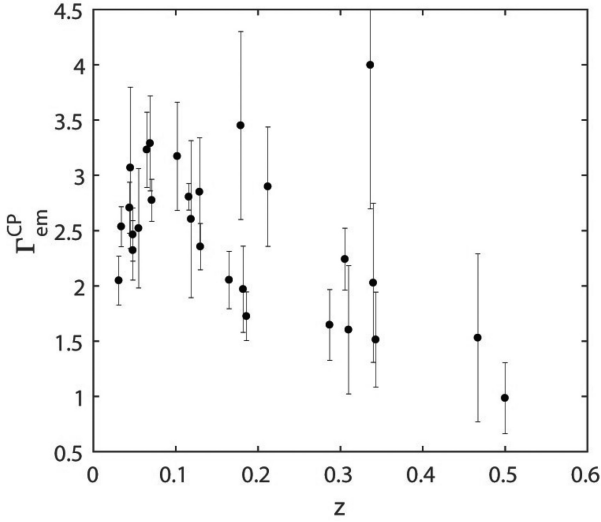
Figure 6. The values of \Gamma_{\text{em}}^{\text{CP}} with the corresponding error bars are plotted versus z for all blazars in S_0 .
