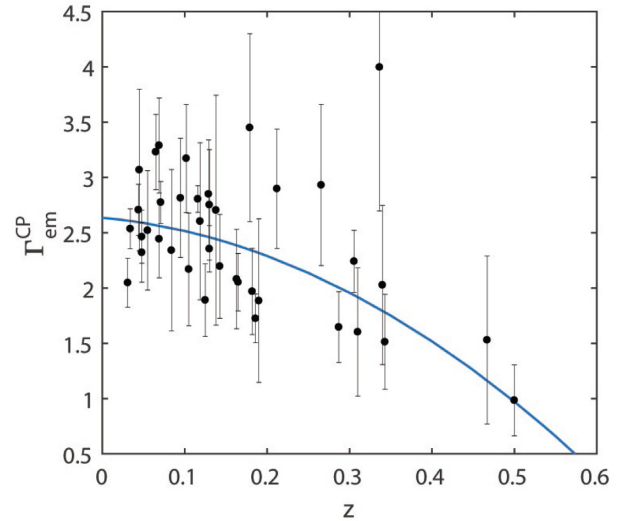
Figure 3. Same as Fig. 2, but with superimposed the best-fitting regression line with \chi^2_{\text{red,CP}} = 1.46 .
