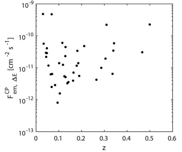
Figure 8. The values of F_{\text{em},\Delta E}^{\text{CP}} are plotted versus z for all blazars of S .
