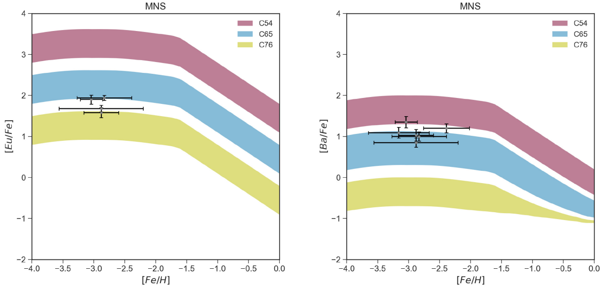
Figure 10. Results of models C54, C65, and C76 for Reticulum II for [\text{Eu}/\text{Fe}] and [\text{Ba}/\text{Fe}] versus [\text{Fe}/\text{H}] in the case of one event of MNS in the first Gyr.
