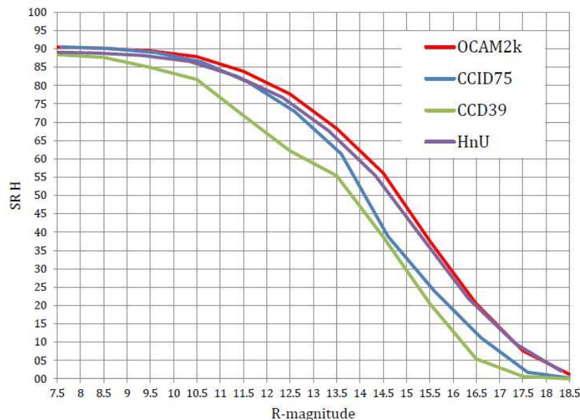
Figure 2: the SOUL improvement in the LBT AO performance (the current is in green line) with different CCD choices, computed with a seeing of 0.8'' . The baseline for SOUL is the OCAM2K camera.
