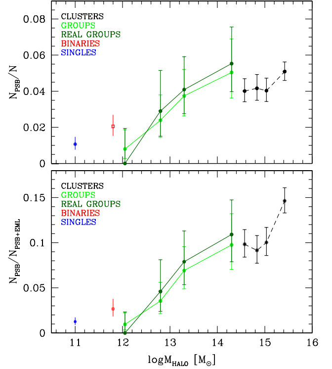
Figure 8. Fraction of PSB galaxies with respect to the total population (upper panel) and with respect to the active population (EML + PSB, lower panel) as a function of the halo mass. Black dots and dashed lines represent the cluster data; green (dark green) dots and solid lines represent the PSB fractions in groups (real groups). The red empty square and the blue point at \log(M_{\text{halo}}/M_{\odot}) = 11.8 and 11 show the value for binaries and single galaxies, respectively. Errors are binomial.
