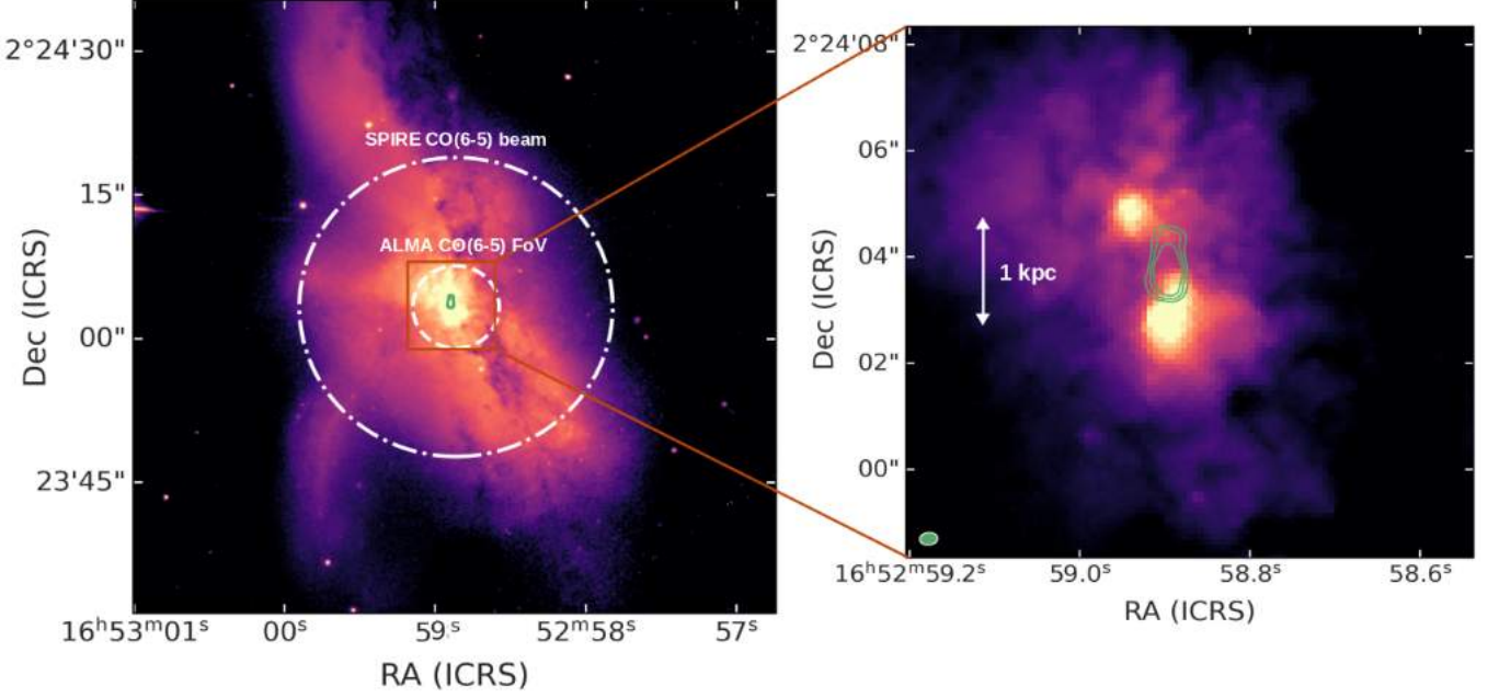
Figure B5. Left panel: HST WFC2 F814W image of NGC 6240 (from Gerssen et al. 2004 ), with superimposed, in green, the contours of ALMA CO(6–5) moment 0 at the resolution of 250 mas (project 2015.1.00658.S, PI: Rangwala). The contours are drawn at (3, 4, 5, 10, 20) \times \sigma , where \sigma = 29 \text{ Jy beam}^{-1} \text{ km s}^{-1} . The inner white dashed circle indicates the FoV of both ALMA observations, with a radius of 4''.3 ( \sim 2.1 \text{ kpc} ), while the outer dash-dotted circle represents the Herschel /SPIRE-FTS beam FWHM for CO(6–5) observations, with a 15''.6 radius. Right panel: zoom of the inner 4.5 kpc. The restored ALMA beam is shown as a green ellipse with white edges at the bottom left.
