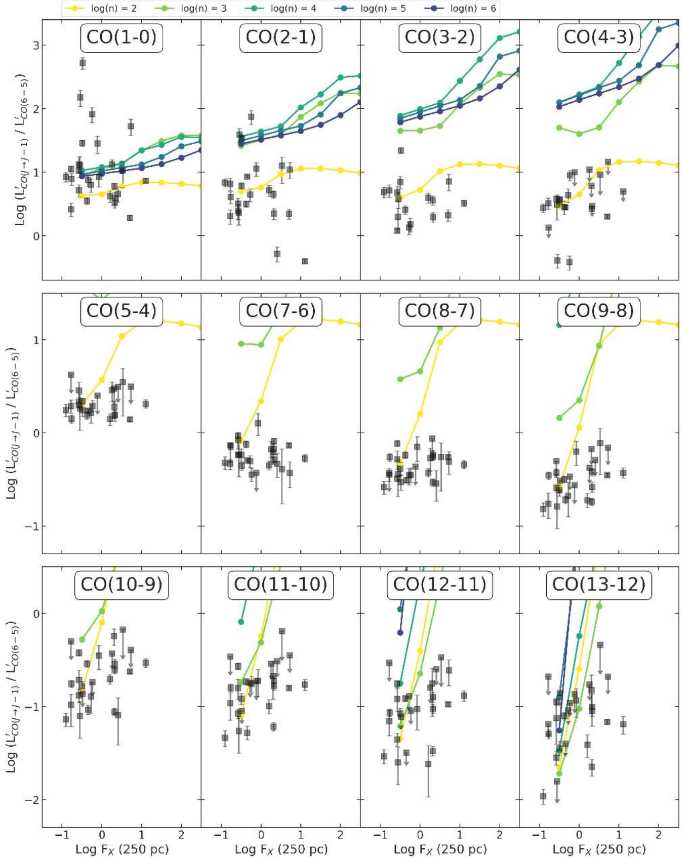
Figure A8. CO line ratios, with respect to the CO(6–5) line, vs. F_X . The x-axis is F_X (for r = 250 pc), in units of \text{erg s}^{-1} \text{cm}^{-2} . The y-axis is the luminosity ratio L'_{\text{CO}(J \rightarrow J-1)} / L'_{\text{CO}(6-5)} to the CO(6–5) line. Data points and lines are described in Figure A5.
