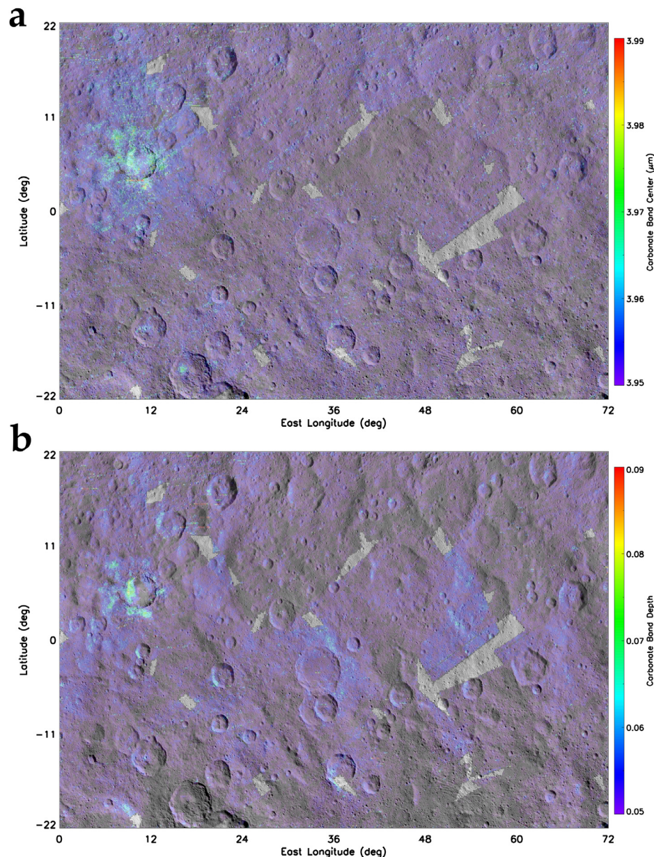
Fig. 11. Distribution of 4.0- \mu\text{m} band's center (a) and band depth (b) values across quadrangle Ac-H-6 Haulani, derived from VIR data. These parameters are respectively sensitive to the composition and abundance of carbonate minerals. The overall distribution spans from Mg- or (Mg,Ca)-rich carbonates (violet to blue) to Na-rich carbonates (red) (a), and from lower depth (violet to blue) to greater depth (red) (b). Local enhancement of Ca-rich and possibly Na-rich carbonates is found locally in the region of crater Haulani, most notably in its western inner wall and ejecta closest to the southern rim. Other evidences of Ca-rich carbonates are found in part of Kondos crater's floor and in the ejecta of a fresh unnamed crater located at 20.7^{\circ}\text{N}/7.6^{\circ}\text{E} , even though with smaller concentrations compared to crater Haulani. (For interpretation of the references to color in this figure legend, the reader is referred to the web version of this article.)
