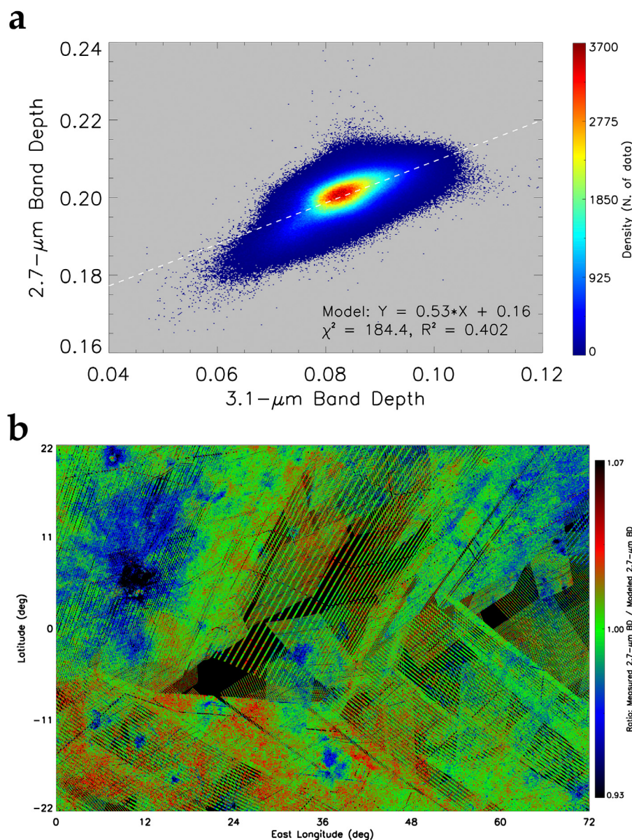
Fig. 8. a: Density scatterplot of 2.7-μm band depth (BD27) as a function of 3.1-μm band depth (BD31) computed for the quadrangle Ac-H-6. A linear fit model (white dashed line) is superimposed on the distribution (values of the chi-square ( \chi^2 ) and the coefficient of determination (i.e., the squared correlation coefficient R^2 ) are also provided). Most data concentrate around the average values. The cluster shows a large spread and a moderate-to-low correlation in the linear fit model. b: Ratio between the measured 2.7-μm band depth and the BD27/BD31 linear fit model. This map shows where the surface material departs from an ideally linear correlation between the abundance of the two major mineral species. Dark blue to blue colors mark locations that have shallower BD27 than the linear model, while red to dark red shades mark locations that have larger BD27 than the linear model. If BD27 was perfectly correlated with BD31, this map would appear uniformly green. In the map, disconnected lines within a given image are due to the high instantaneous speed of the ground footprints (i.e., projections of the spectrometer's slit) in the HAMO phase. (For interpretation of the references to color in this figure legend, the reader is referred to the web version of this article.)
