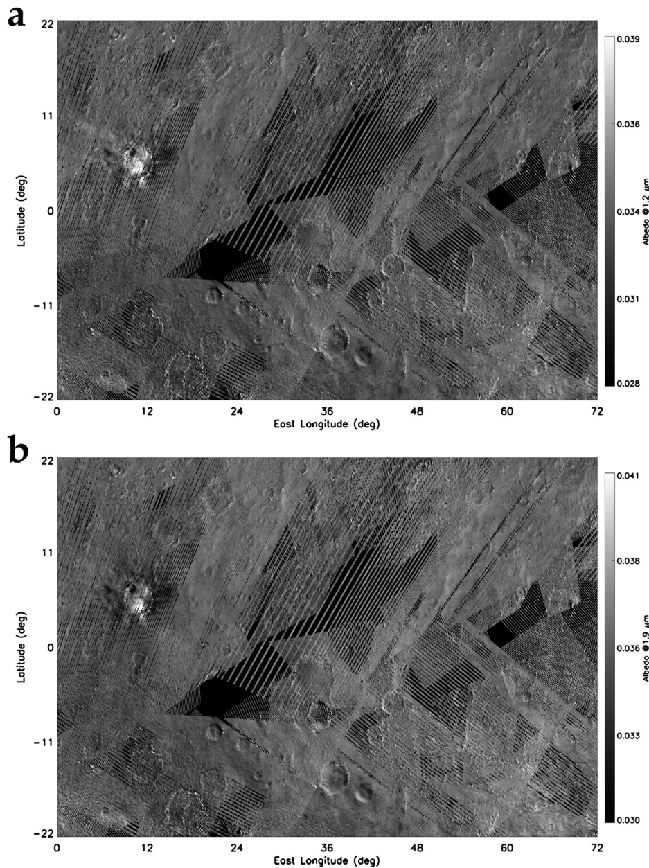
Fig. 3. a: Reflectance map of Ac-H-6 Haulani, obtained through photometric correction of VIR data acquired at 1.2\mu\text{m} in the Survey and HAMO mission phases, interpolated on a grid with a fixed resolution of \sim 140\text{ m/pixel} , photometrically corrected by using the method described by Ciarniello et al. (2017), i.e. a Hapke photometric correction to standard observation geometry ( i = 30^\circ , e = 0^\circ , \alpha = 30^\circ ). b: Reflectance map of Ac-H-6 Haulani, obtained through photometric correction of VIR data acquired at 1.9\mu\text{m} in the Survey and HAMO mission phases, interpolated on a grid with a fixed resolution of 140\text{ m/pixel} . The same photometric correction of (a) was applied. In both maps, disconnected lines within a given image are due to the high instantaneous speed of the ground footprints (i.e., projections of the spectrometer's slit) in the HAMO phase.
