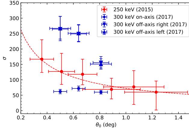
Fig. 9 Best fit values of \sigma of the 2017 data sets, compared with the previous values for the incident energy of 250 keV (see Fig. 5). Error bars on the values of \sigma at 95%.
