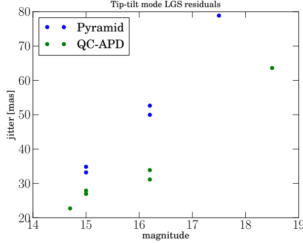
Figure 3. Comparison of the quad-cell APD with the pyramid WFS, both used as tip-tilt sensors. The comparison is performed in daytime with atmospheric turbulence emulated on the secondary mirror. The jitter is measured here from the LGS wavefront sensor tip-tilt residuals. While it may be an optimistic prediction with respect to nighttime condition due to low vibration level, this comparison suggests that the QC APD tip-tilt sensor brings an improvement of more than a magnitude with respect to the pyramid.
