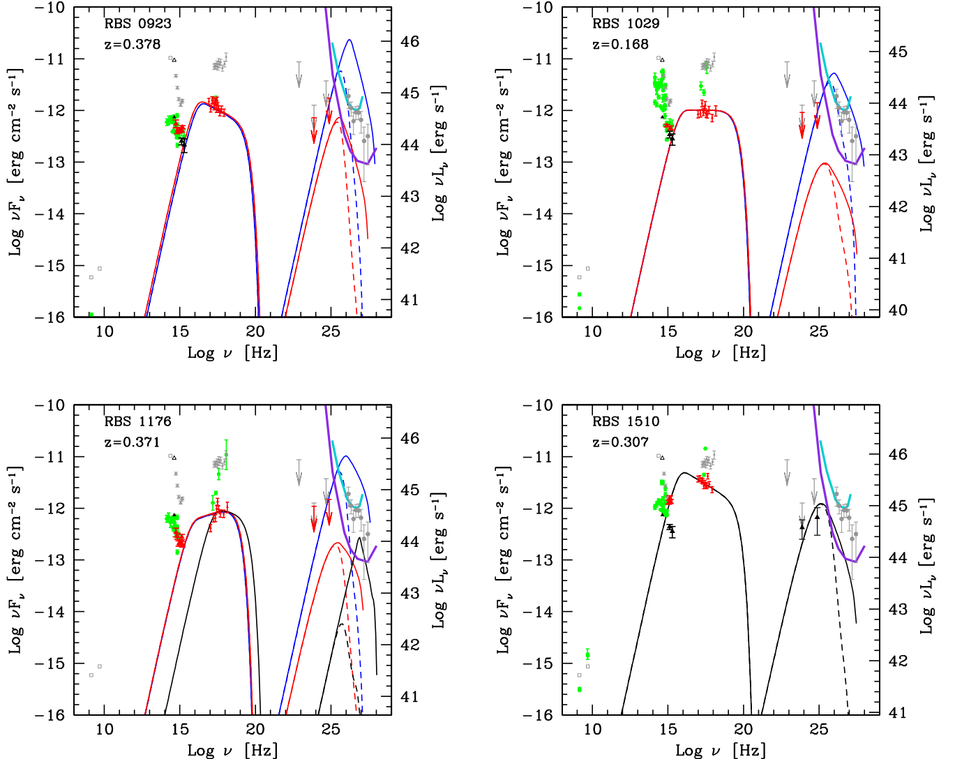
Figure 4. As in Fig. 3. In the case of RBS 1176, the black line refers to the model assuming the highest value of \gamma_{\min} compatible with the X-ray spectrum ( \gamma_{\min} = 4 \times 10^5 , see Table 6).
