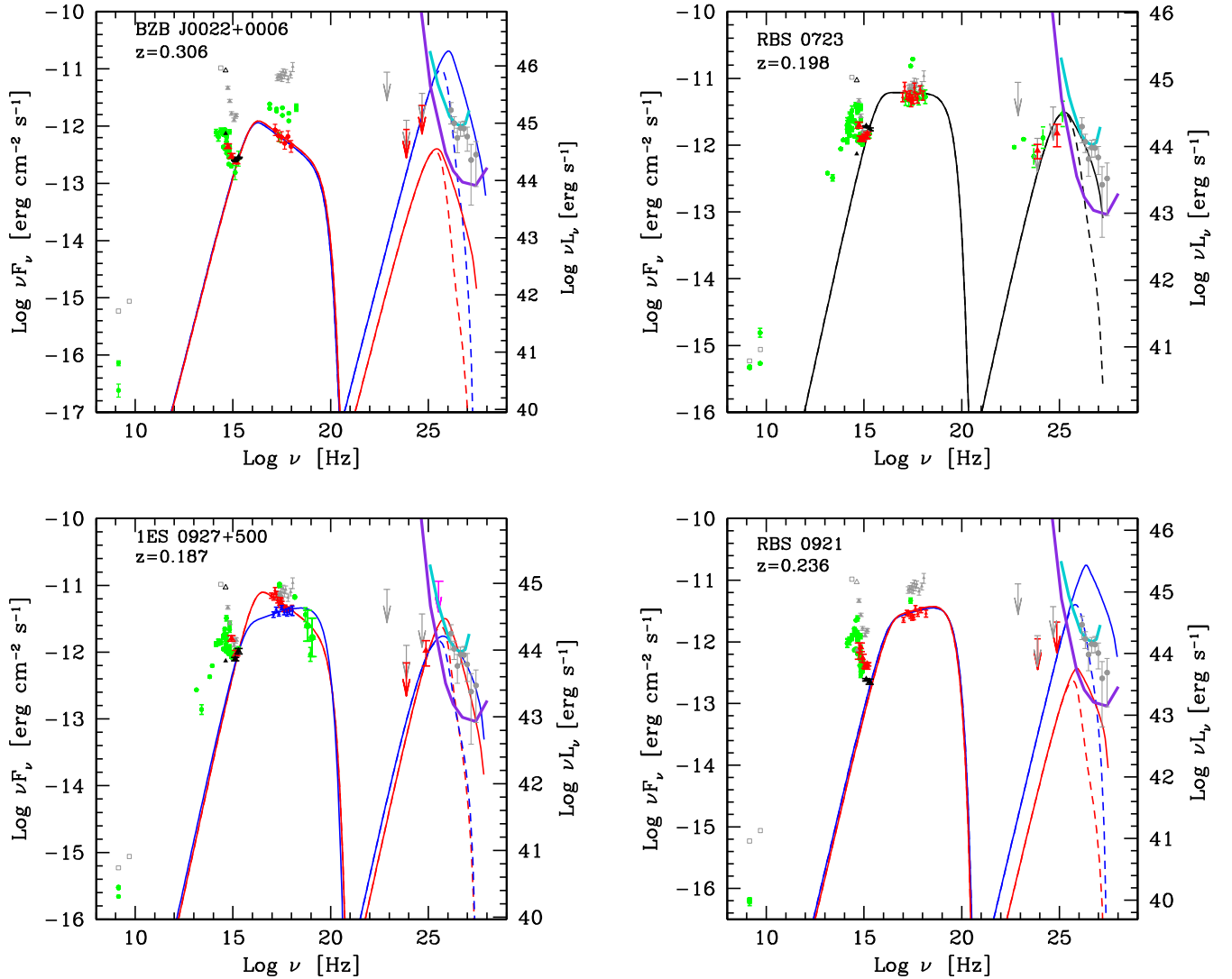
Figure 3. SED of the selected extreme BL Lac objects. Green symbols reports historical data from ASI/ASDC archive. Red symbols show Swift /UVOT, XRT, and Fermi /LAT data discussed in the text. Black symbols display GALEX data. Background grey symbols show the SED of 1ES 0229+200 for comparison. For sources not detected by LAT, we report two different models of the SED, corresponding to low ( B = 0.01 G, blue lines) and high ( B = 0.1 G, red lines) magnetic field. For sources with a LAT detection we only report one model, in black (parameters are reported in Table 6). For 1ES 0927+500 we report two models, corresponding to the two X-ray slopes (see Table 2). Dashed lines show the model after absorption with the EBL, calculated according to Domínguez et al. (2011). Light blue and violet curves report the differential sensitivities ( 5\sigma , 50 h of exposure, 5 bins per energy decade) of MAGIC and CTA, respectively.
