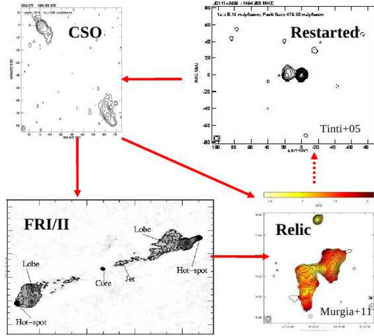
Fig. 3 The evolutionary path of the radio emission. Young CSO ( top left , image adapted from Orienti et al. 2004) may become either a classical large FRII ( bottom left , image adapted from Mack et al. 2009) or a relic in the case of the activity phase switches off soon after its onset ( bottom right , image adapted from Murgia et al. 2011). If the central engine goes through another active phase, a newly-born bright and compact object can be observed close to the relic of the previous activity ( top right , image adapted from Tinti et al. 2005).
