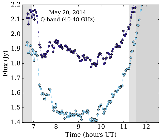
Figure 4. Higher-frequency Q-band (43 GHz) observation (dark blue points) for the 2014 May 20 light curve (left panel) and the light curves for both the K-band (23 GHz) and Q-band normalized by the phase calibrator light curve (right panel). As in Figure 1, the phase calibrator is represented by the light blue points and the K-band light curve by the purple points.
