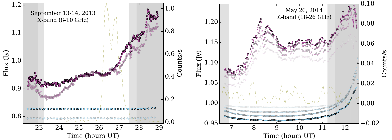
Figure 3. Frequency dependence of two radio flares. The darker curves are the highest frequencies, and the lighter curves represent progressively lower frequencies for each observation. Note the dip in the lower-frequency bands for Sgr A* around UT 23–24. The two light curves meet just before the strong X-ray flare.
