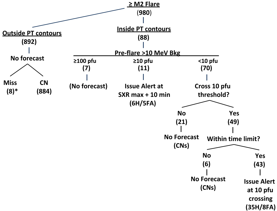
Figure 4. Decision tree for ESPERTA forecasts of \geq S2 SPEs (1995–2014). PT—prediction threshold; CN—correct null; H—Hit; FA—False Alarm. The symbol * indicates that there are six other misses (MISSes in Table 2) from visible disk flares that did not reach the M2 level. Four other \geq S2 events were associated with < M2 flares from behind the solar limb.
