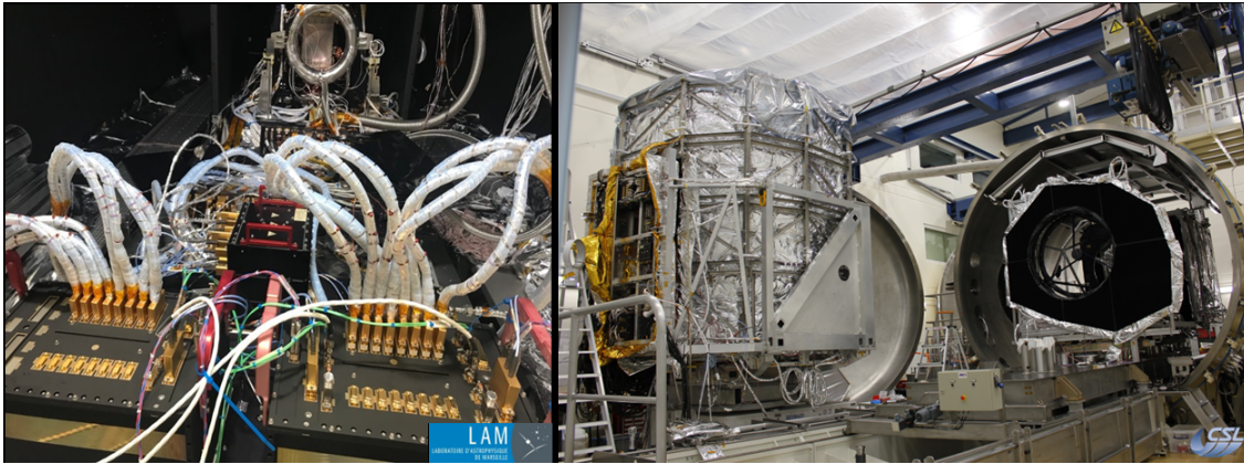
Figure 8. Left : NISP tests setup at Laboratoire d'Astrophysique di Marseille , France. NISP warm electronics close-up, from bottom to top: the two DPUs, the ICU, and the focal plane array. Right : Euclid's end-to-end PLM test setup at the Centre Spatial de Liège , Belgium. The NISP warm electronics mounted on the pannel Y can be seen at the left-side of the picture (vertical structure partially covered with MLI), and the telescope placed horizontally at the right-side of the image.
