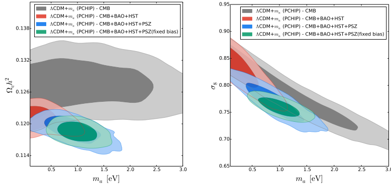
Fig. 7. 68% and 95% CL allowed regions in the (m_a, \Omega_c h^2) plane (left panel) and in the (m_a, \sigma_8) plane (right panel) for different data combinations, when a PCHIP PPS is assumed. From Ref. [94].
