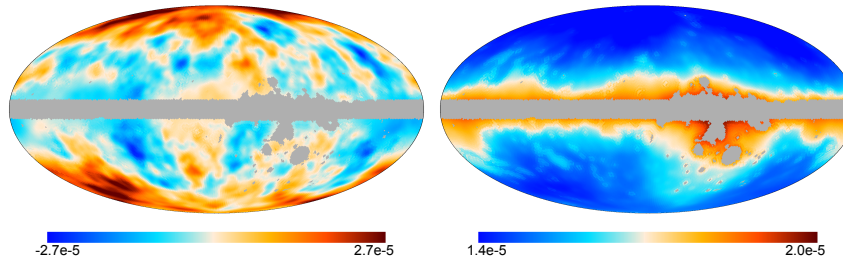
Fig. 1. Map (thermodynamic temperature in K) of the recovered ISW anisotropies (left) and its corresponding estimated error per pixel (right), from the combination of the Planck SEVEM CMB map and all the LSS tracers. The error map structure is determined by the sky coverage of the different surveys. The total signal-to-noise of the ISW map cannot exceed, obviously, a value of \approx 4 . The signal-to-noise is higher near the Galactic poles, with values of \approx 2 .
