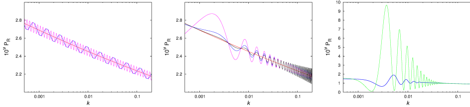
Fig. 4. PPS simulated for various oscillatory models parametrized with an amplitude, a frequency and a phase (for the Linear oscillation models we have the scale-dependence index as further parameter). Left: Log-spaced oscillations models for different values of the frequency oscillation parameter. Middle: Linear oscillation models for different values of the scale-dependence index. Right: Step oscillation models for different values of the frequency and phase parameters.
