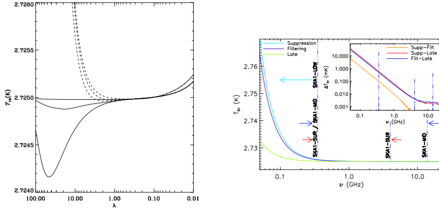
Fig. 9. Left panel: distorted spectra in equivalent thermodynamic temperature vs. \lambda (cm) with late energy injection \Delta\epsilon/\epsilon_i = 5 \times 10^{-6} plus an early/intermediate energy injection \Delta\epsilon/\epsilon_i = 5 \times 10^{-6} ( \sim 20 times smaller than current upper limits) at the “time” Comptonization parameter y_h = 5, 1, 0.01 (bottom to top; the cases at y_h = 5 and 1 are very similar at short \lambda ; solid lines) plus a FF distortion with y_B = 10^{-6} (dashes). y_h = y with T_e = T_{CMB} when the integral is computed from the energy injection time to the current time. Right panel: FF distortion in SKA2 frequency range by two astrophysical reionization histories (a late phenomenological model is also displayed for comparison). Inset: models absolute differences; vertical lines: ranges of SKA1 configurations. From Ref. [141].
