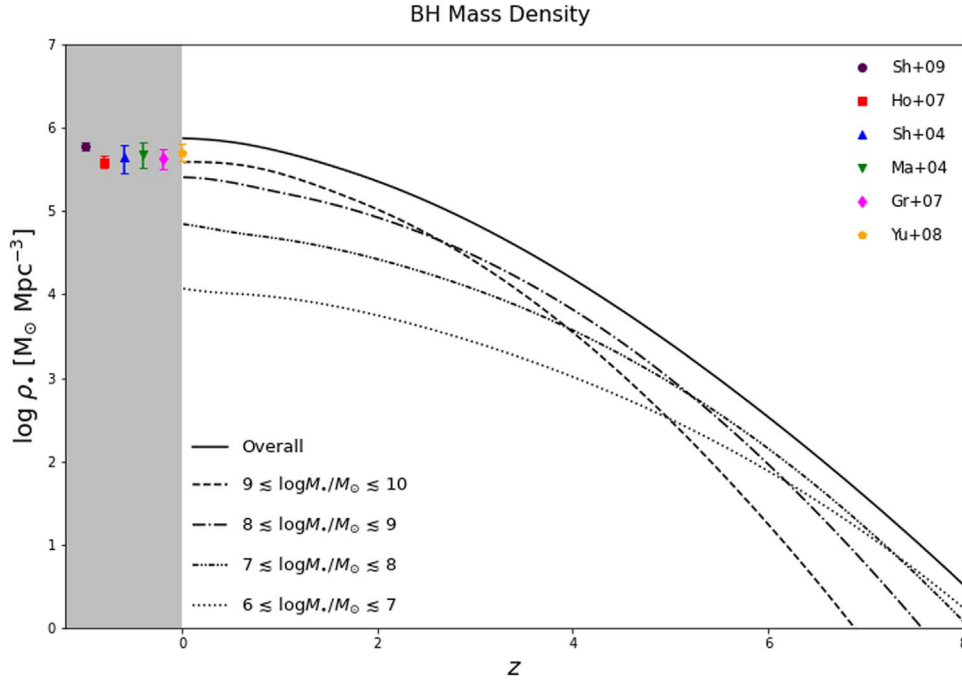
Figure 8. The (super)massive relic BH mass density (see Equation (20)) as a function of redshift z . The overall mass density is illustrated (solid) together with the contributions from the mass ranges 10^6 M_\odot \lesssim M_* \lesssim 10^7 M_\odot (dotted), 10^7 M_\odot \lesssim M_* \lesssim 10^8 M_\odot (triple-dotted-dashed), 10^8 M_\odot \lesssim M_* \lesssim 10^9 M_\odot (dotted-dashed), and 10^9 M_\odot \lesssim M_* \lesssim 10^{10} M_\odot (dashed). Observational estimates at z \approx 0 are from Shankar et al. (2009; brown circle), Hopkins et al. (2007; red square), Shankar et al. (2004; blue triangle), Marconi et al. (2004; green inverted triangle), Graham et al. (2007; magenta diamond), and Yu & Lu (2008; orange pentagon).
