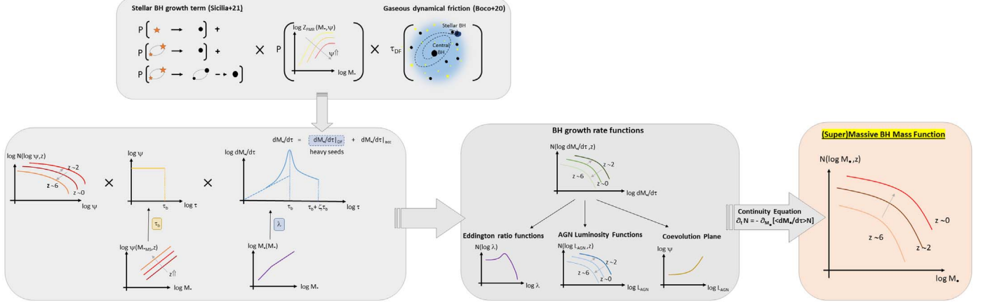
Figure 1. Schematics showing the main steps to compute the (super)massive relic BH mass function. The starting point is the stellar term from Paper I, representing the number of BHs originated per unit of star formed mass, and includes contributions from the evolution of isolated or binary stars into isolated or binary BHs (light seeds; see Equation (5)). This is coupled with the metallicity distribution (extracted from the fundamental metallicity relation) and the timescale for gaseous dynamical friction by Boco et al. (2020; see Equation (A1)) to derive the growth rate of the central BH by migration of stellar remnants (see Equations (7) and (8)). In parallel, galaxy statistics provided by the SFR functions are coupled with model growth curves of the stellar and BH mass (see Equations (2) and (13)); the latter includes the growth by dynamical friction migration and gaseous Eddington-type accretion. The crucial parameters of these growth curves, like the star formation duration and Eddington factor, are derived by requiring consistency with the main sequence of star-forming galaxies (see Equations (3) and (4)) and the local Magorrian relationship (see Equations (14) and (15)). The main outcomes of this procedure are BH growth rate functions (see Equation (16)), and the by-products are Eddington ratio functions, AGN luminosity functions (Equation (18)), and the coevolution plane SFR vs. L_{\text{AGN}} . Finally, a generalized continuity equation approach allows one to convert the growth rate functions into the (super)massive BH mass function (Equation (19)).
