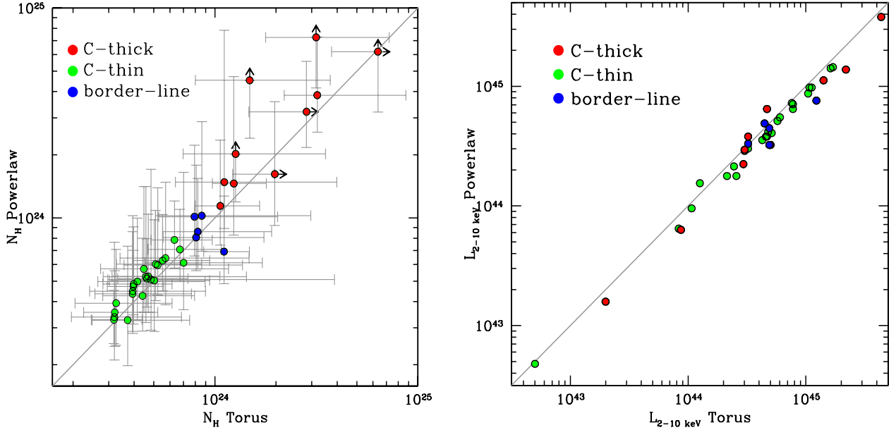
Fig. B.1. Left panel: comparison of the N_H best fit obtained from the PI ( y -axis) and Tor ( x -axis) models. Right panel: comparison of the 2–10 keV, absorption corrected luminosity, obtained from the same two models. In both panels we show CTN i sources in green, CTK i sources in red and border-line sources in blue, and the solid line represents the 1:1 relation.
