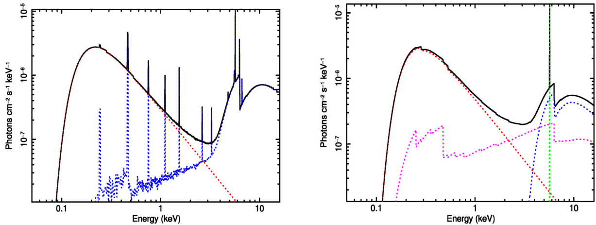
Fig. 3. As an example, the two models used in the fit of source 2608 at z = 0.125 are shown: Tor (left) and PI (right). In the Tor model the blue line includes the primary power-law, the reflection component and fluorescence lines, all self-consistently computed as a function of N_H and geometry. In the PI model the blue line represents the primary power-law, modified by photoelectric absorption and taking into account Compton scattering (PLCABS component in Xspec). The magenta line represents the PEXRAV component (i.e. reflection produced by a slab of infinite optical depth material), and the green line represents a Gaussian emission line reproducing the fluorescent Fe K \alpha line. In both models the red line represents the secondary power-law, reproducing scattered light and/or thermal emission in the soft band.
