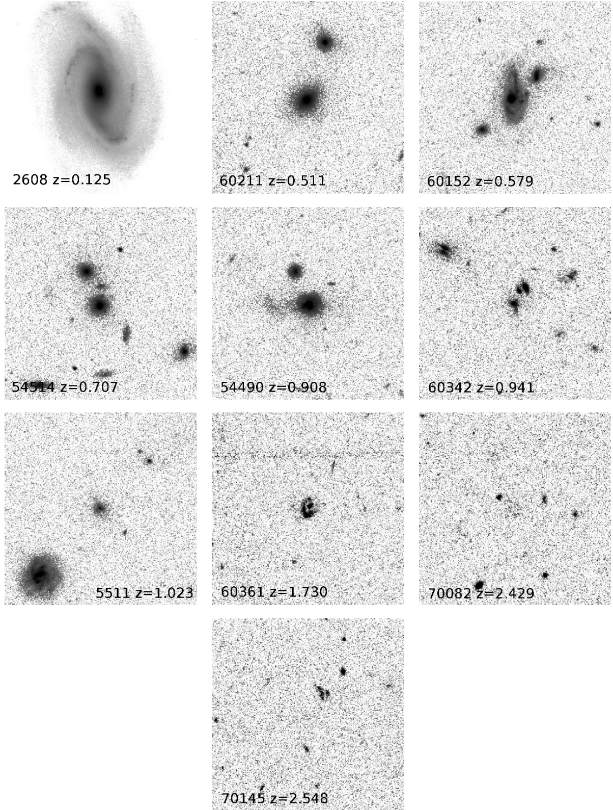
Fig. 12. HST-ACS I band 15'' × 15'' cut-outs of the COSMOS mosaic (Koekemoer et al. 2007), for the ten CTK f sources, ordered by increasing redshift.
