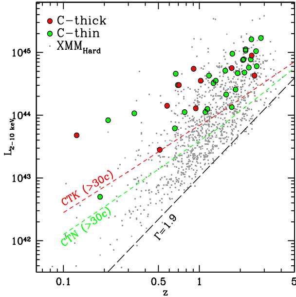
Fig. A.1. Redshift vs. L_{2-10} distribution for CTK f (red) and CTN f (green) sources. Gray squares represent the 2–10 keV band detected XMM-COSMOS sources. The black dashed line represents the detection limit computed for an unabsorbed power-law with \Gamma = 1.9 , while the red (green) dashed line show the detection limit computed for a CTK (CTN) source.
