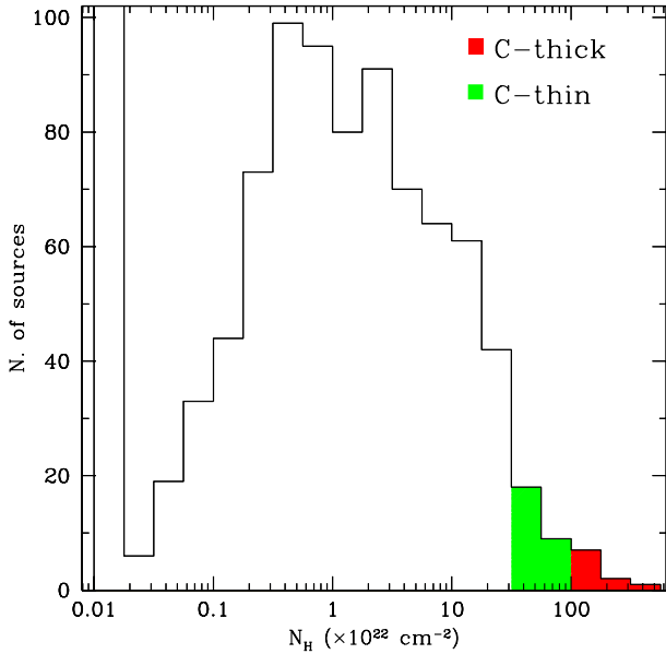
Fig. 1. Distribution of N_H (in units of 10^{22} \text{ cm}^{-2} ) in the XMM-COSMOS survey. Only extragalactic sources with >30 pn net counts are shown. The green (red) shaded histogram show the sample of \text{CTN}_i ( \text{CTK}_i ) sources. The first bin includes the 390 sources for which the N_H is an upper limit (for clarity the y -axis is rescaled in the range 0–100).
