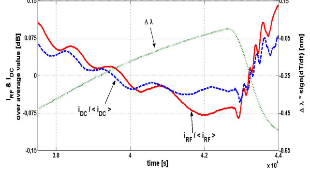
Figure 6: Measured behavior in dB of i_{DC} (dashed line) and i_{RF} (continuous line), referred to their respective average values, versus time. The values of \Delta\lambda over time (dotted line) are represented as well. See text for details.
