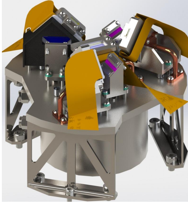
Figure 8. Interior of the detector vacuum chamber showing almost all focal plane components: LGMLs (magenta), CCD faces (blue), and flex prints (gold). A black anodized CCD baffle with a horizontal rectangular aperture restricts the view of the CCDs to its LGML.
