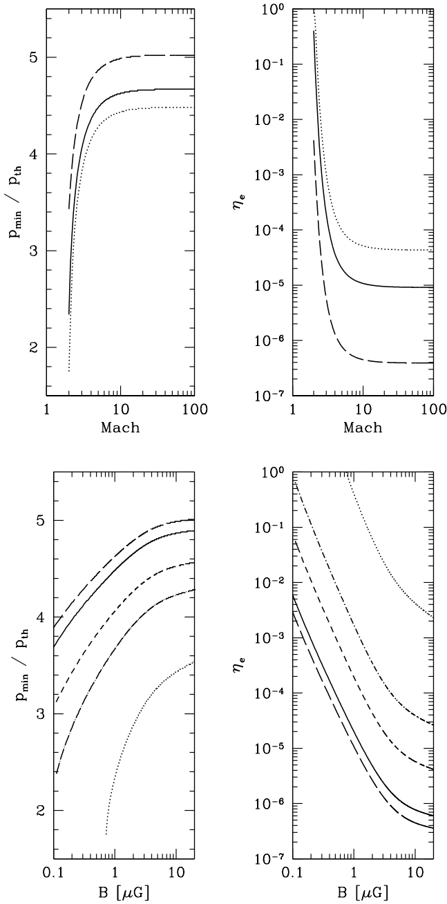
Fig. 2. Values of p_{\min}/p_{\text{th}} and \eta_e for a mock radio relic (see text) at fixed magnetic field ( top ) and Mach number ( bottom ). Top panels: curves denote different values of B : 0.5 \mu\text{G} (dotted), 1 \mu\text{G} (solid) and 10 \mu\text{G} (dashed). Bottom panels: curves denote different values of M : 2 (dotted), 2.5 (dot-dashed), 3 (short dashed), 5 (solid) and 10 (long dashed).
