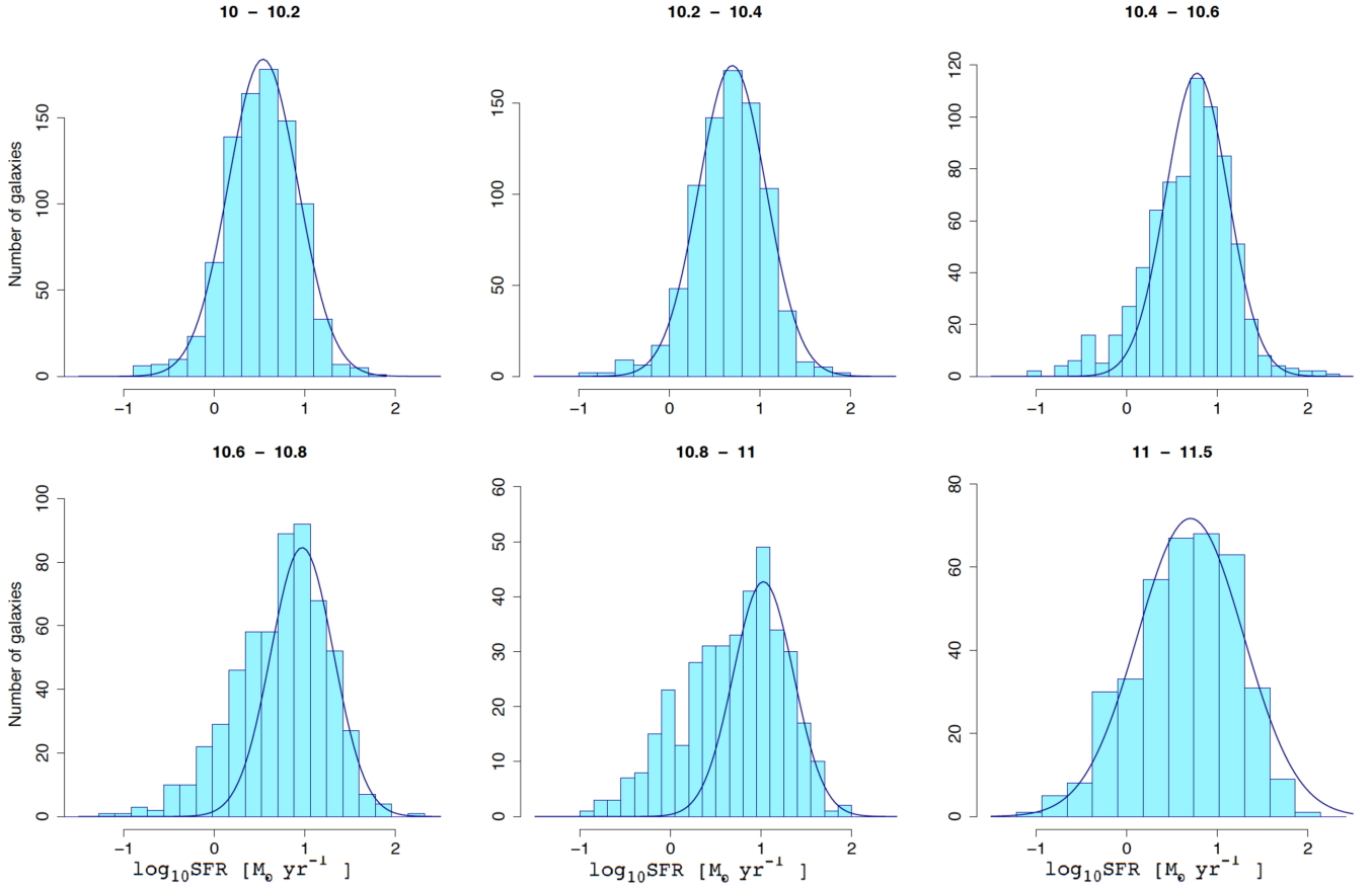
Figure 2. Distribution of SFR of all IR-detected galaxies at 0.15 < z < 0.5 in different stellar mass bins.
