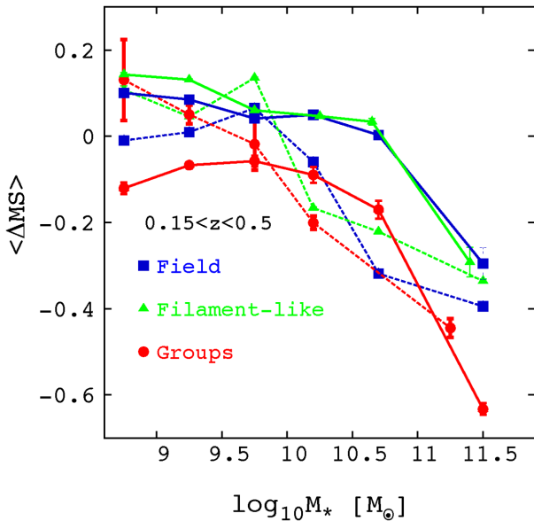
Figure 10. The MS offset for field, ‘filament-like’ and group star-forming galaxies as a function of stellar masses in the low redshift bin for disc-dominated ( n_{\text{Sérsic}} < 2 with solid lines) and bulge-dominated galaxies ( n_{\text{Sérsic}} > 2 with dashed lines).
