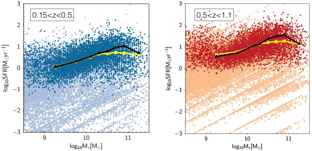
Figure 4. Left-hand panel: SFR versus M_* for galaxies in 0.15 < z < 0.5 . The dark blue points show the IR-detected galaxies and the light blue points show galaxies with \text{SFR}_{\text{SED}} . The black connected triangles show the peak of distribution of SFR in different mass bins for IR-detected galaxies and the yellow connected circles show the mean of SFR for IR-detected galaxies. Right-hand panel: same as left-hand panel for galaxies in 0.5 < z < 1.1 .
