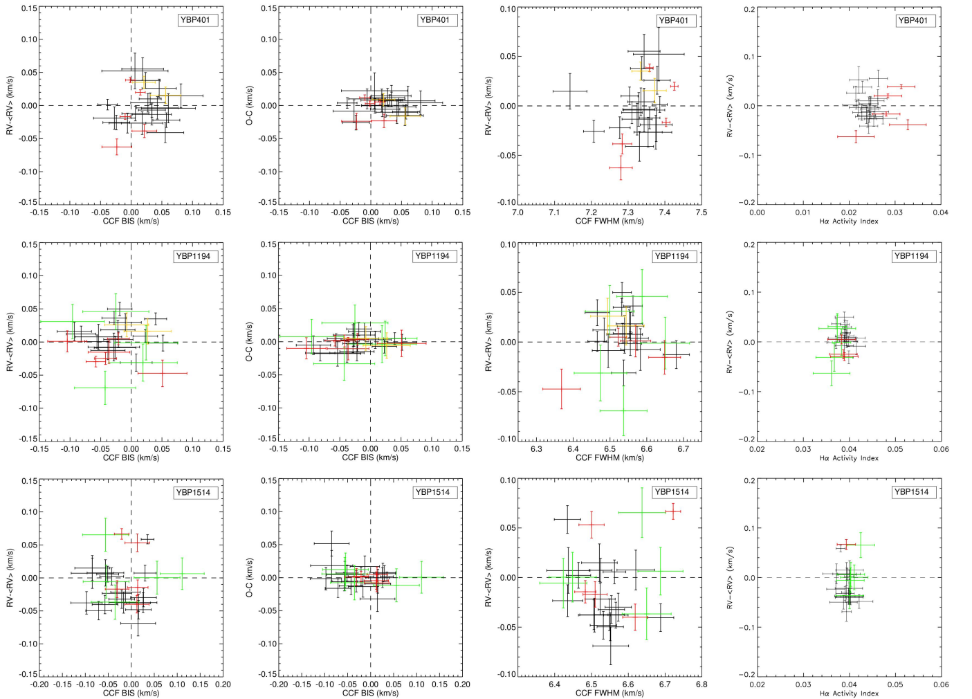
Fig. A.2. Top: RV measurements versus bisector span, residuals versus bisector span, RV measurements versus CCF FWHM and RV measurements versus H\alpha activity indicator for YBP401. The H\alpha activity indicator is computed as the area below the core of H\alpha line with respect to the continuum. CCF FWHM values are calculated by subtracting the respective instrumental FWHM in quadrature. Same symbols as in Fig. 2. Middle: the same plots for YBP1194. Bottom: the same plots for YBP1514.
