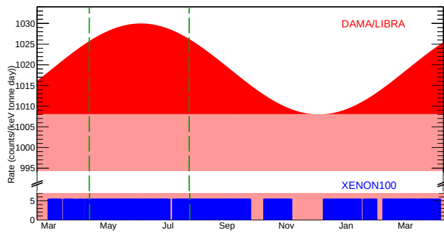
FIG. 1: Conceptual illustration of the analysis. Shown is the DAMA/LIBRA rate (red) [20] with the modulated rate in (2 - 6) keV from the fit parameters in [4] (dark red). The distribution of the XENON100 live time (blue) is indicated with its average background rate of 5.3 \text{ events}/(\text{keV} \cdot \text{tonne} \cdot \text{day}) , which shows dents due to maintenance or calibration campaigns. The region between the dashed lines (green) indicates the 70 summer live days where the modulated signal is expected to be largest.
