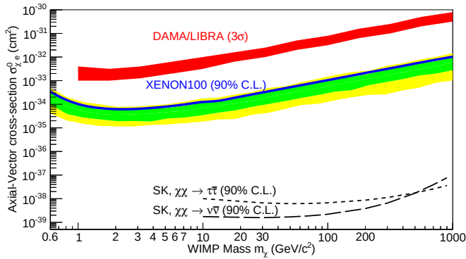
FIG. 4: Parameter space for WIMPs coupling to electrons through axial-vector interactions. The XENON100 upper limit (90% confidence level) is indicated by the blue line, along with the green/yellow bands indicating the 1\sigma/2\sigma sensitivity. For comparison, we also show the DAMA/LIBRA allowed region (red) and the constraint from Super-Kamiokande (SK) using neutrinos from the Sun, by assuming dark matter annihilation into \tau\bar{\tau} or \nu\bar{\nu} , both calculated in [11].
