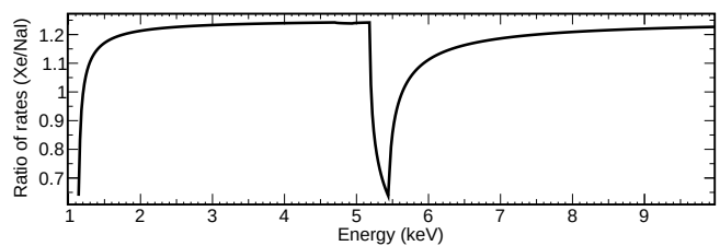
FIG. 2: Calculated ratio of the differential rates in xenon and sodium iodide for inelastic WIMP-electron scattering through axial-vector coupling. The structures around 1 and 5 keV are owing to the small difference in the binding energies of the 3s and 2s shells in xenon and iodine.
