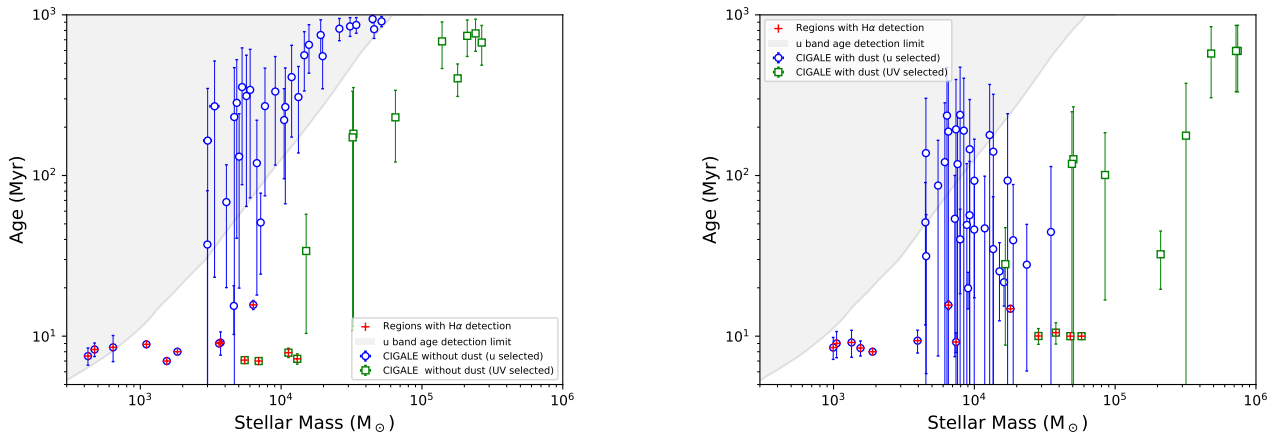
Fig. B.1. Age and stellar mass determined using CIGALE for all the regions in Table 3. These panels can be directly compared to Fig. 9 obtained with Starburst99. Left and right panels: results obtained with CIGALE without and with dust, respectively. The blue circles and green squares represent u -band- and UV-selected regions, respectively. The gray shaded area is our u -band detection limit in stellar mass and age. The red crosses identify the H\alpha detected regions.
