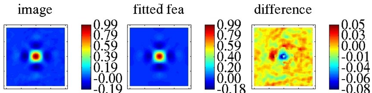
Figure 6. Comparison between the VLT-DSM IF measured on the test bench and Finite Element Model, sampled at the 3x3 actuator scale. The RMS difference is < 2% for most of the actuators, largely due to convection noise in the measurement.
