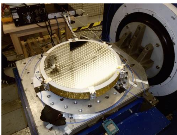
Figure 9. The TS was installed on a vibration test platform and exposed to a launch acceleration spectrum, while the ES locking was engaged. The TS survived the test, proofing the effectiveness of the EL concept.
