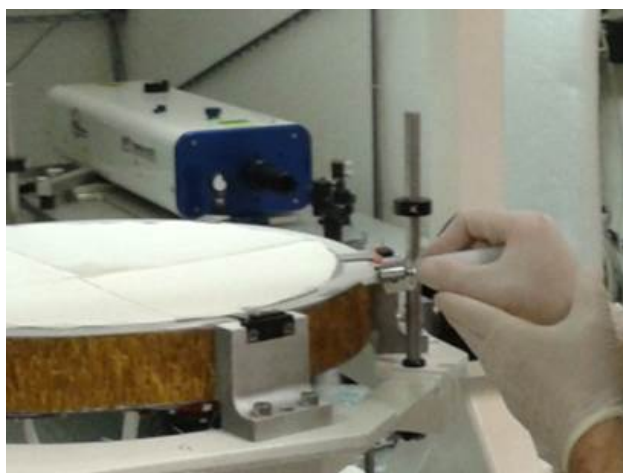
Figure 8. Electrostatic Locking test: an electrical field is applied to the TS to lock into the RB. During the test the adhesive force was measured by pushing laterally the TS to check the detaching force.
